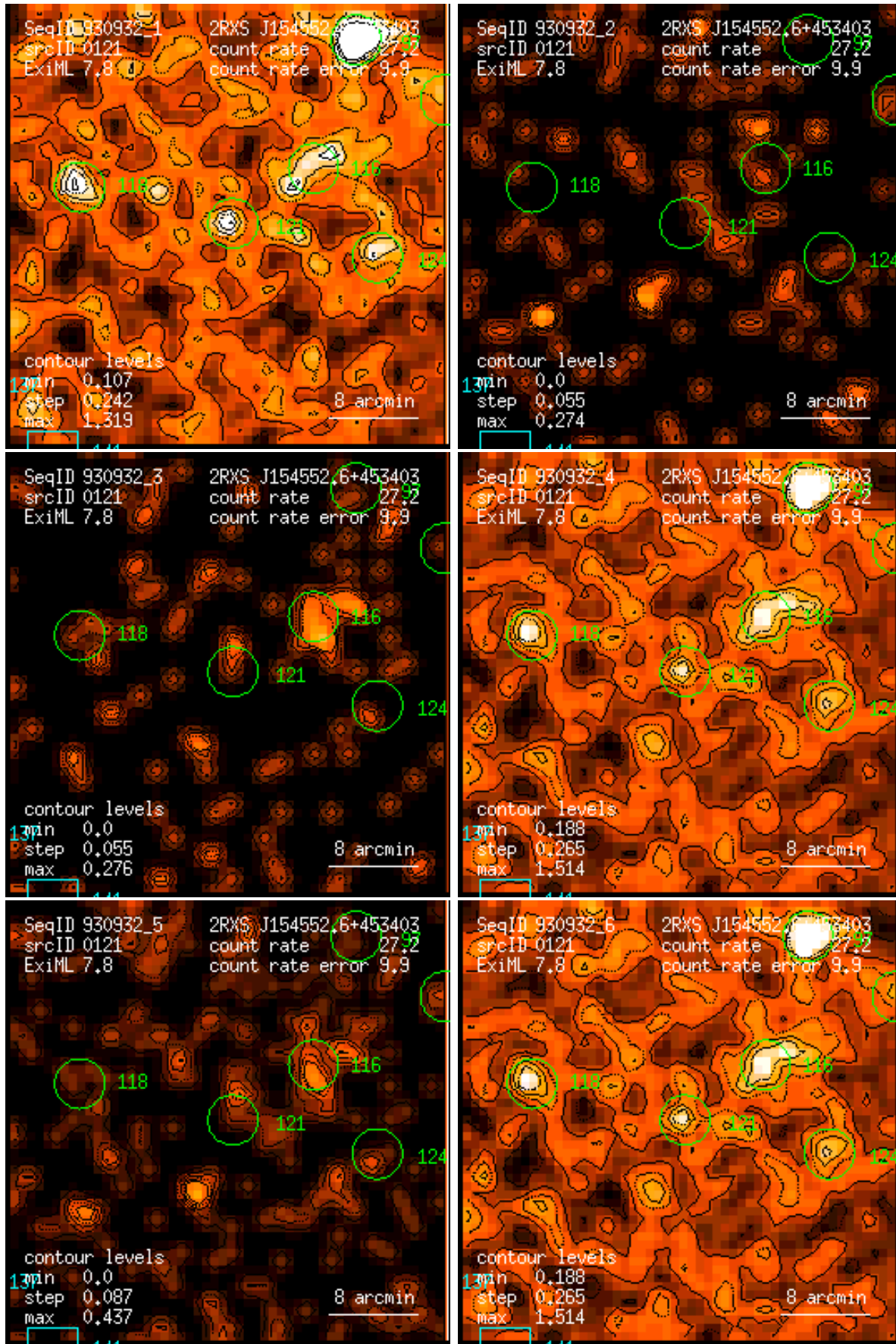
Figure 121: RASS 930932: detection 0121: band rate images, Gaussian filter: (1) PSPC channels 11 – 41, (2) 52 – 90, (3) 91 – 201, (4) 11 – 235, (5) 52 – 201, (6) 11 – 201. Broad band rates in counts/ks. Band rate contour levels in counts/ks/arcmin 2 .
