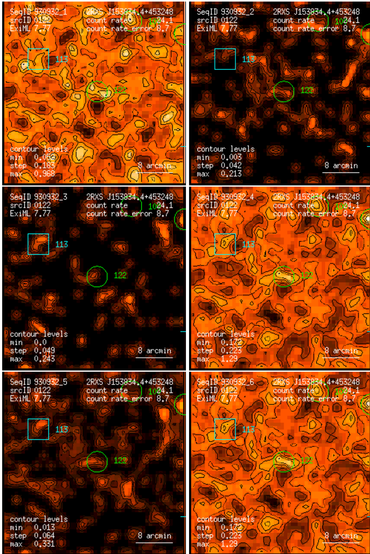
Figure 122: RASS 930932: detection 0122: band rate images, Gaussian filter: (1) PSPC channels 11 – 41, (2) 52 – 90, (3) 91 – 201, (4) 11 – 235, (5) 52 – 201, (6) 11 – 201. Broad band rates in counts/ks. Band rate contour levels in counts/ks/arcmin 2 .
