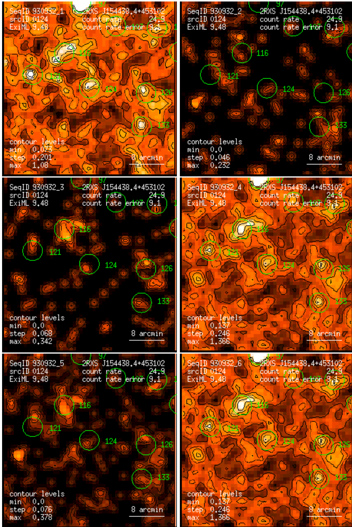
Figure 124: RASS 930932: detection 0124: band rate images, Gaussian filter: (1) PSPC channels 11 – 41, (2) 52 – 90, (3) 91 – 201, (4) 11 – 235, (5) 52 – 201, (6) 11 – 201. Broad band rates in counts/ks. Band rate contour levels in counts/ks/arcmin 2 .
