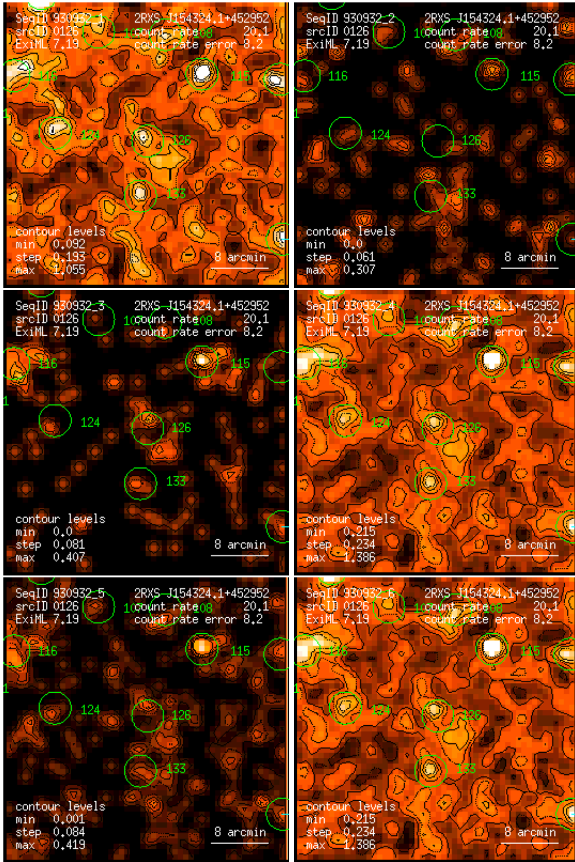
Figure 126: RASS 930932: detection 0126: band rate images, Gaussian filter: (1) PSPC channels 11 – 41, (2) 52 – 90, (3) 91 – 201, (4) 11 – 235, (5) 52 – 201, (6) 11 – 201. Broad band rates in counts/ks. Band rate contour levels in counts/ks/arcmin 2 .
