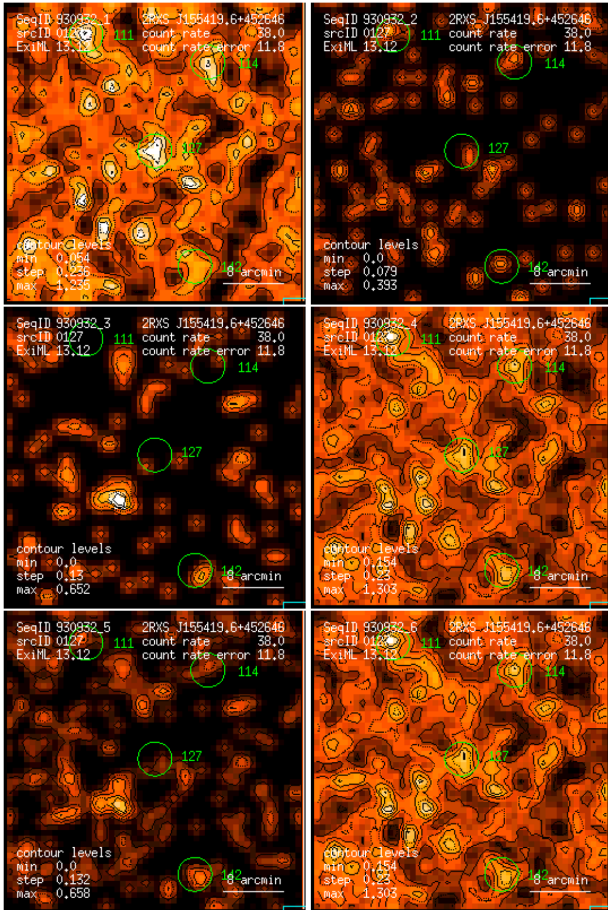
Figure 127: RASS 930932: detection 0127: band rate images, Gaussian filter: (1) PSPC channels 11 – 41, (2) 52 – 90, (3) 91 – 201, (4) 11 – 235, (5) 52 – 201, (6) 11 – 201. Broad band rates in counts/ks. Band rate contour levels in counts/ks/arcmin 2 .
