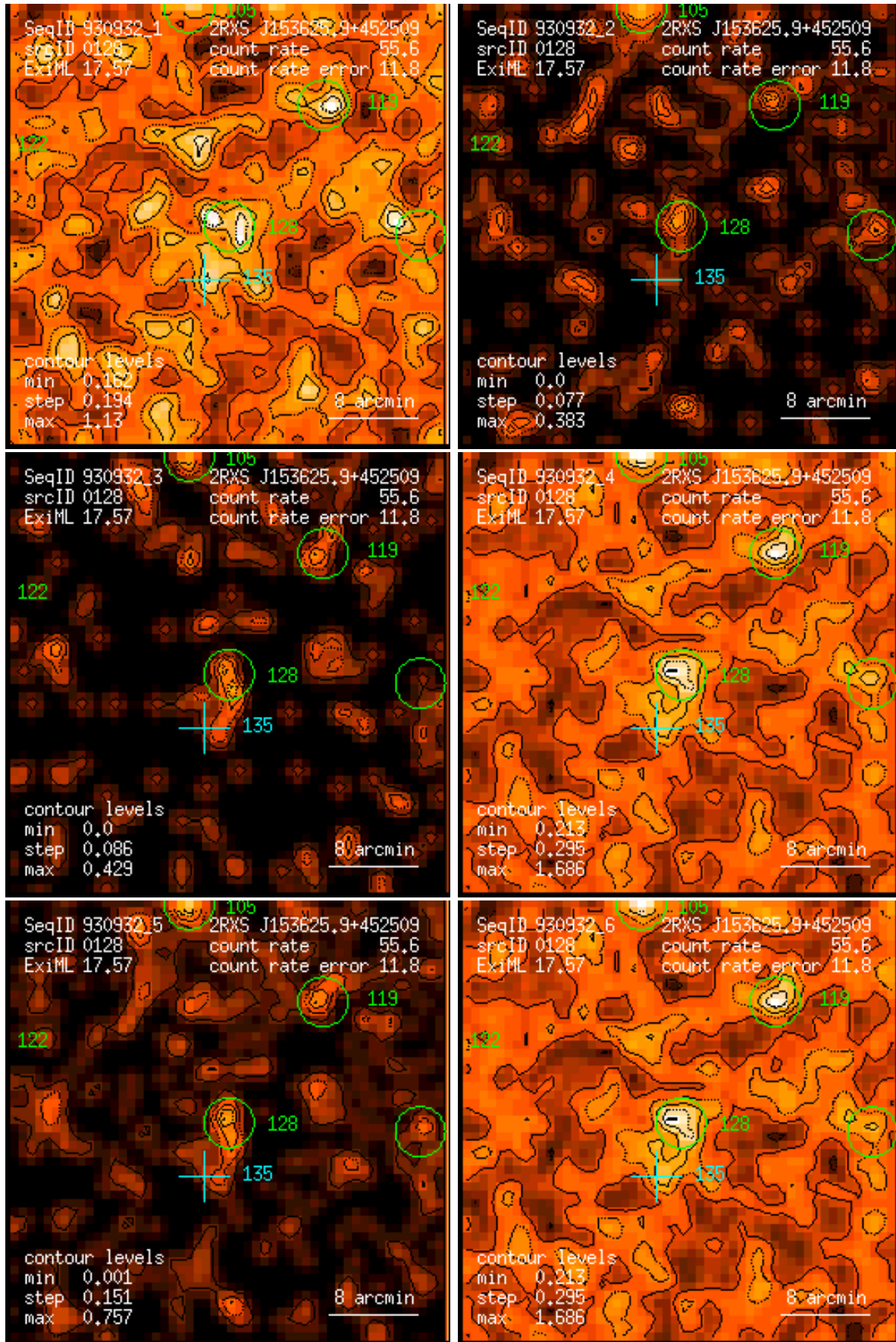
Figure 128: RASS 930932: detection 0128: band rate images, Gaussian filter: (1) PSPPC channels 11 – 41, (2) 52 – 90, (3) 91 – 201, (4) 11 – 235, (5) 52 – 201, (6) 11 – 201. Broad band rates in counts/ks. Band rate contour levels in counts/ks/arcmin 2 .
