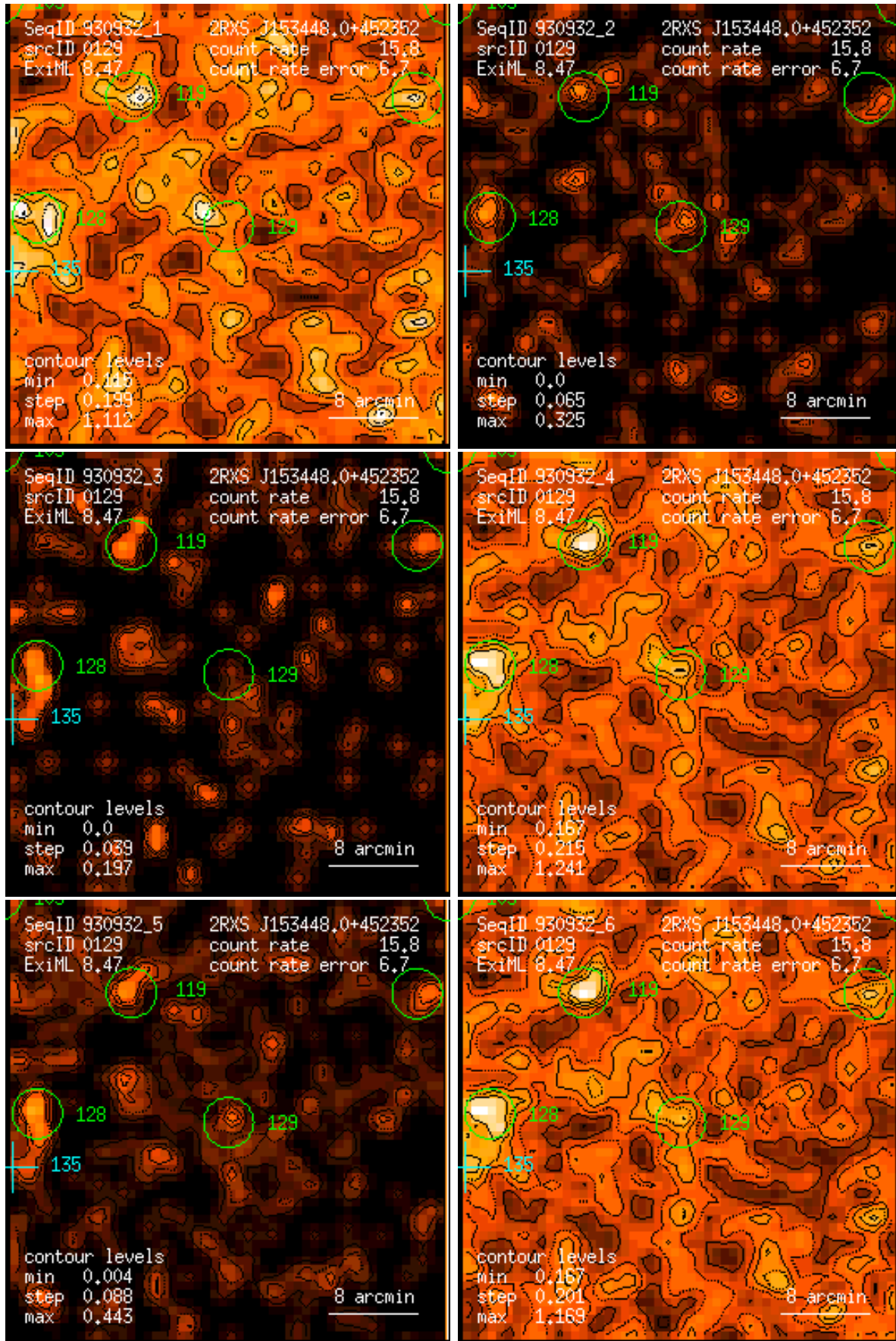
Figure 129: RASS 930932: detection 0129: band rate images, Gaussian filter: (1) PSPC channels 11 – 41, (2) 52 – 90, (3) 91 – 201, (4) 11 – 235, (5) 52 – 201, (6) 11 – 201. Broad band rates in counts/ks. Band rate contour levels in counts/ks/arcmin 2 .
