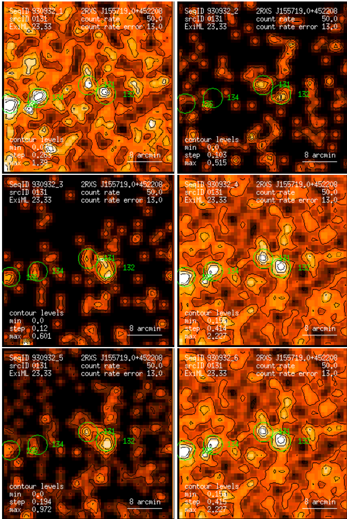
Figure 131: RASS 930932: detection 0131: band rate images, Gaussian filter: (1) PSPC channels 11 – 41, (2) 52 – 90, (3) 91 – 201, (4) 11 – 235, (5) 52 – 201, (6) 11 – 201. Broad band rates in counts/ks. Band rate contour levels in counts/ks/arcmin 2 .
