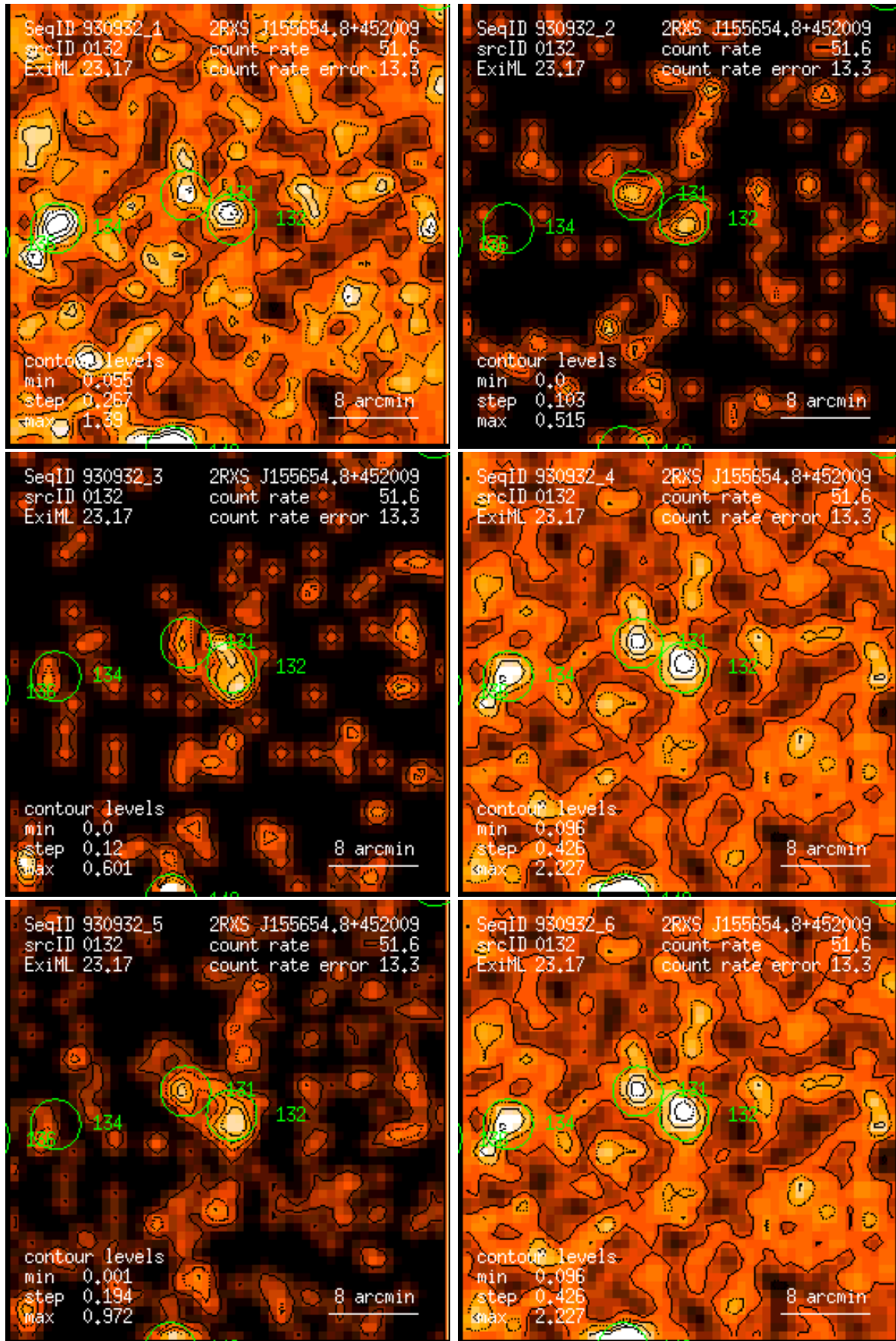
Figure 132: RASS 930932: detection 0132: band rate images, Gaussian filter: (1) PSPC channels 11 – 41, (2) 52 – 90, (3) 91 – 201, (4) 11 – 235, (5) 52 – 201, (6) 11 – 201. Broad band rates in counts/ks. Band rate contour levels in counts/ks/arcmin 2 .
