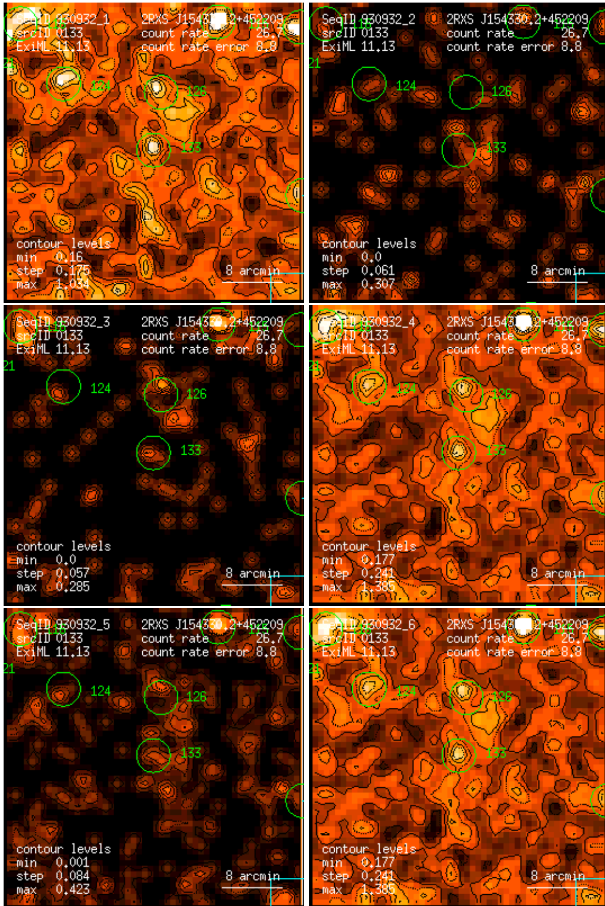
Figure 133: RASS 930932: detection 0133: band rate images, Gaussian filter: (1) PSPC channels 11 – 41, (2) 52 – 90, (3) 91 – 201, (4) 11 – 235, (5) 52 – 201, (6) 11 – 201. Broad band rates in counts/ks. Band rate contour levels in counts/ks/arcmin 2 .
