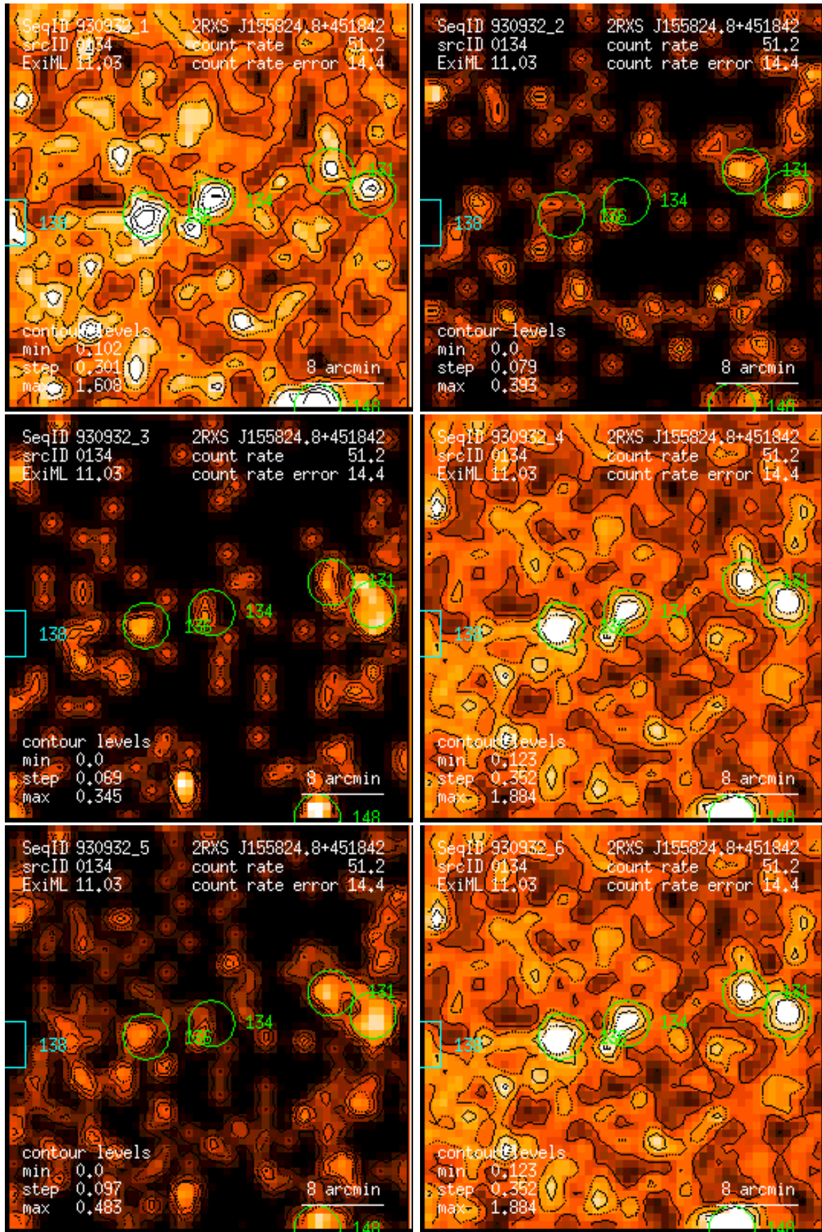
Figure 134: RASS 930932: detection 0134: band rate images, Gaussian filter: (1) PSPC channels 11 – 41, (2) 52 – 90, (3) 91 – 201, (4) 11 – 235, (5) 52 – 201, (6) 11 – 201. Broad band rates in counts/ks. Band rate contour levels in counts/ks/arcmin 2 .
