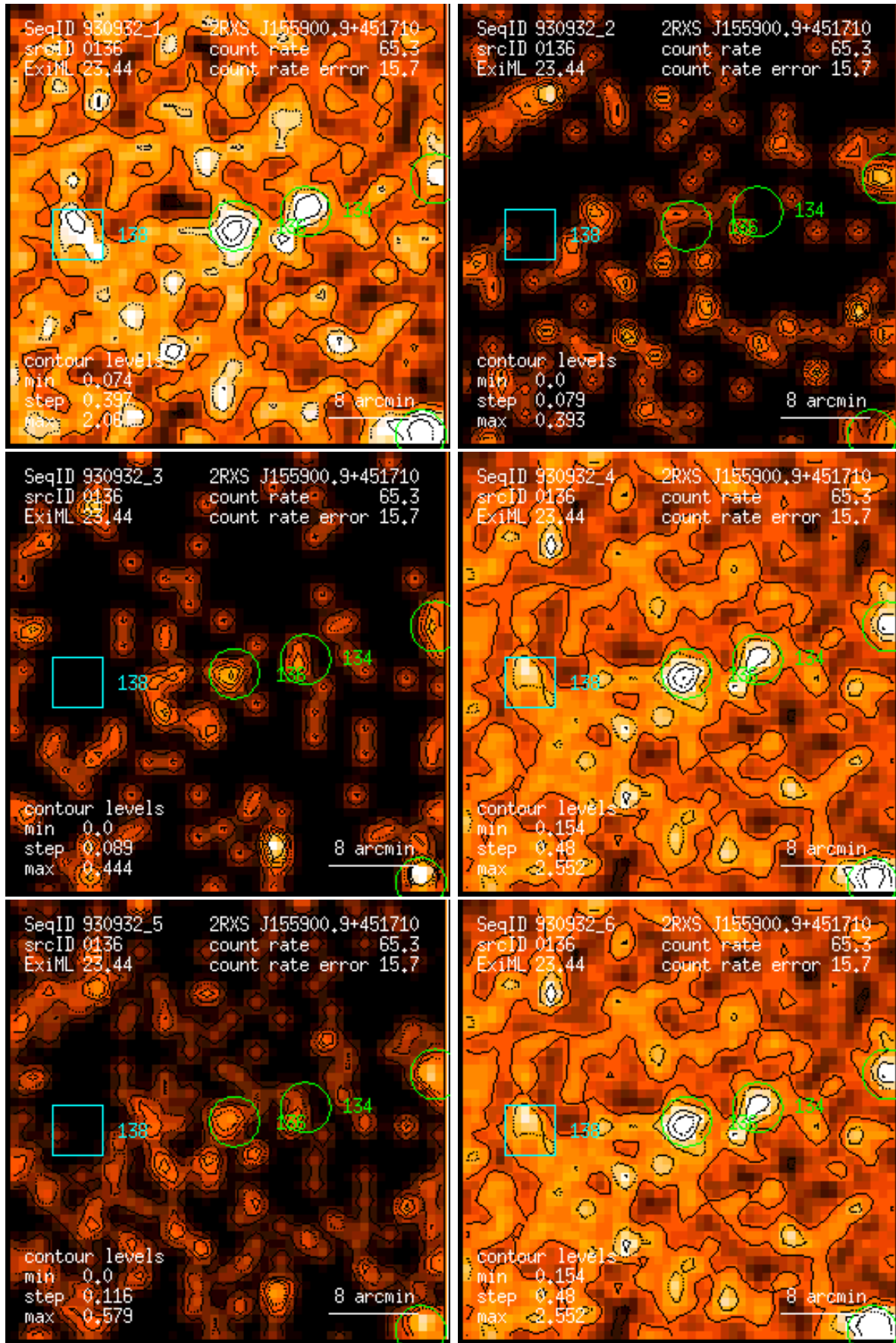
Figure 136: RASS 930932: detection 0136: band rate images, Gaussian filter: (1) PSPC channels 11 – 41, (2) 52 – 90, (3) 91 – 201, (4) 11 – 235, (5) 52 – 201, (6) 11 – 201. Broad band rates in counts/ks. Band rate contour levels in counts/ks/arcmin 2 .
