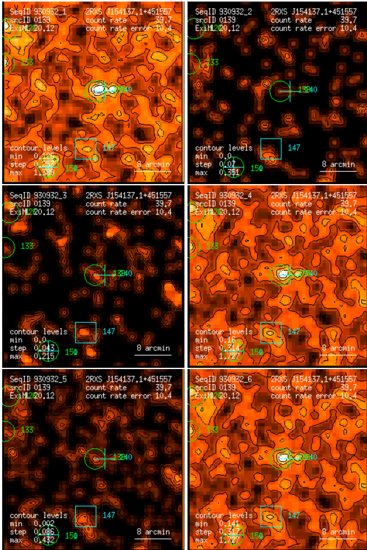
Figure 139: RASS 930932: detection 0139: band rate images, Gaussian filter: (1) PSPC channels 11 – 41, (2) 52 – 90, (3) 91 – 201, (4) 11 – 235, (5) 52 – 201, (6) 11 – 201. Broad band rates in counts/ks. Band rate contour levels in counts/ks/arcmin 2 .
