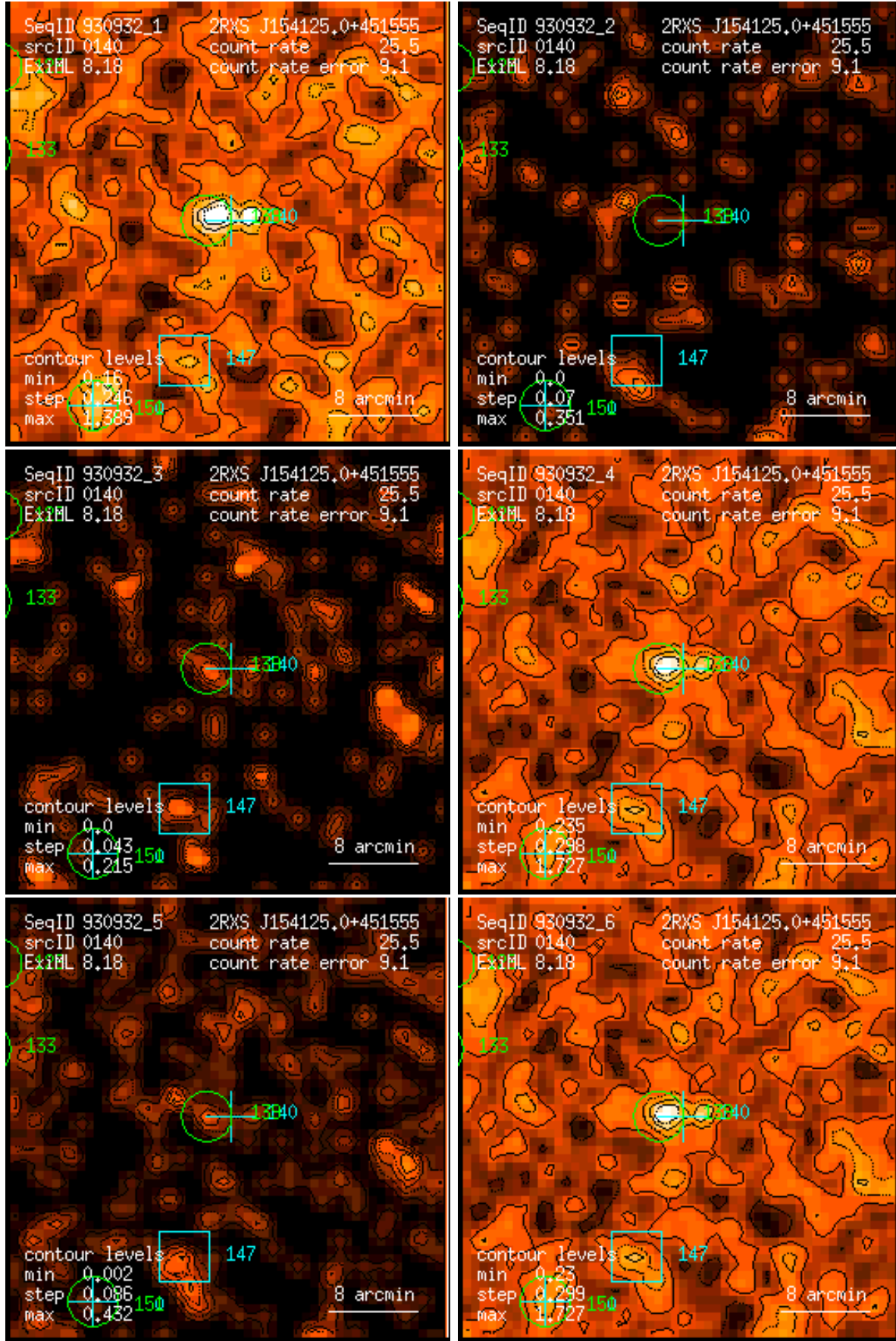
Figure 140: RASS 930932: detection 0140: band rate images, Gaussian filter: (1) PSPC channels 11 – 41, (2) 52 – 90, (3) 91 – 201, (4) 11 – 235, (5) 52 – 201, (6) 11 – 201. Broad band rates in counts/ks. Band rate contour levels in counts/ks/arcmin 2 .
