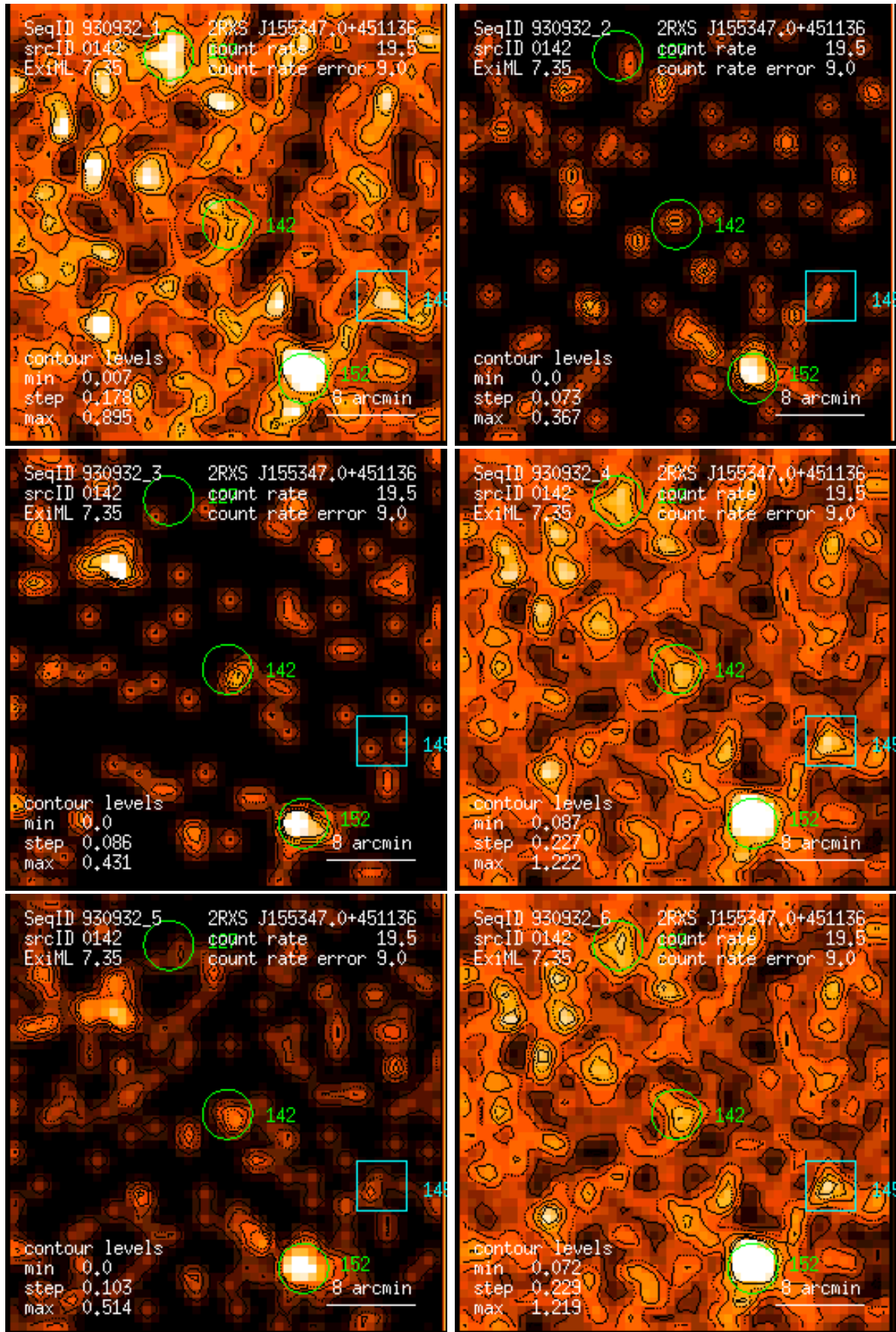
Figure 142: RASS 930932: detection 0142: band rate images, Gaussian filter: (1) PSPC channels 11 – 41, (2) 52 – 90, (3) 91 – 201, (4) 11 – 235, (5) 52 – 201, (6) 11 – 201. Broad band rates in counts/ks. Band rate contour levels in counts/ks/arcmin 2 .
