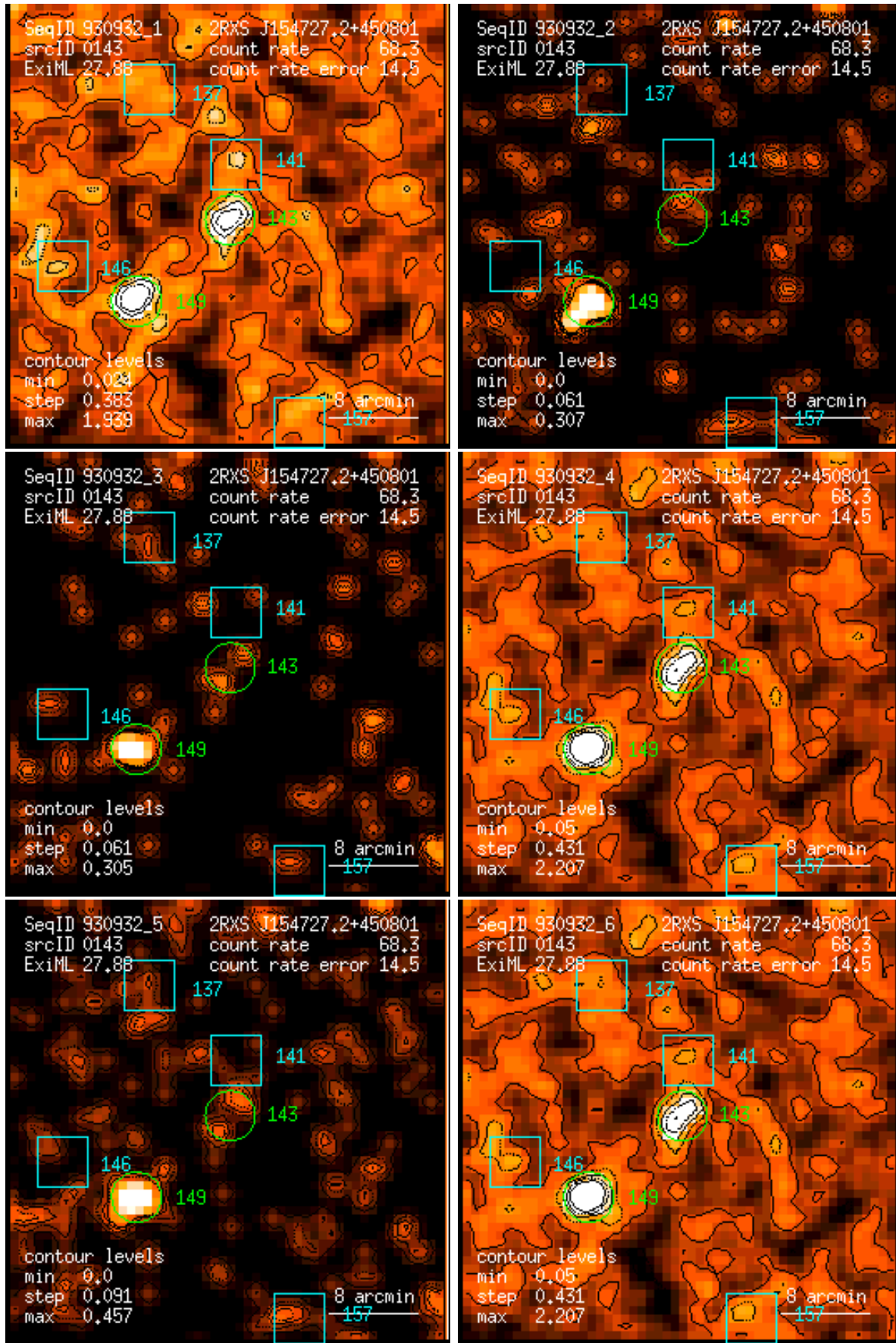
Figure 143: RASS 930932: detection 0143: band rate images, Gaussian filter: (1) PSPC channels 11 – 41, (2) 52 – 90, (3) 91 – 201, (4) 11 – 235, (5) 52 – 201, (6) 11 – 201. Broad band rates in counts/ks. Band rate contour levels in counts/ks/arcmin 2 .
