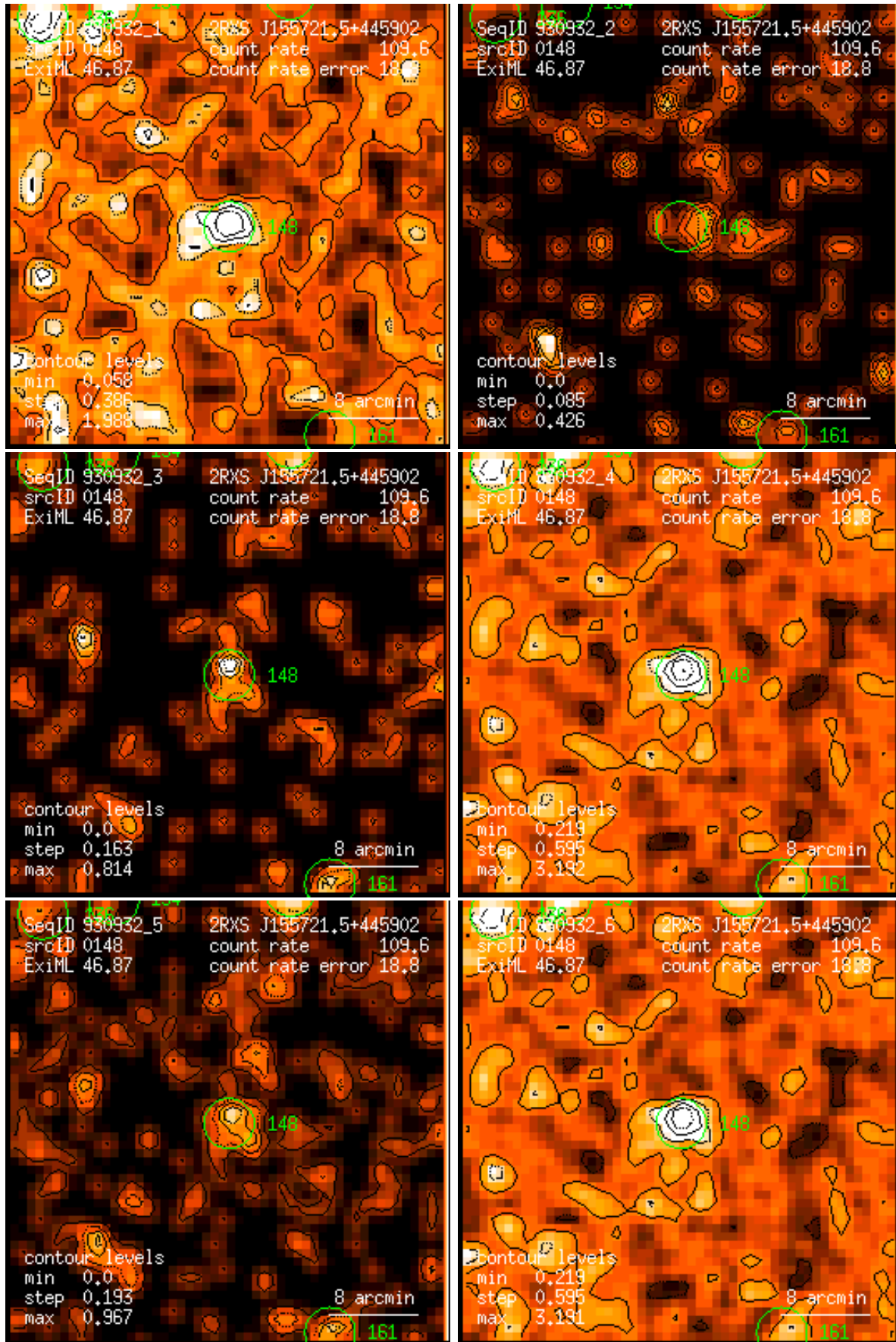
Figure 148: RASS 930932: detection 0148: band rate images, Gaussian filter: (1) PSPC channels 11 – 41, (2) 52 – 90, (3) 91 – 201, (4) 11 – 235, (5) 52 – 201, (6) 11 – 201. Broad band rates in counts/ks. Band rate contour levels in counts/ks/arcmin 2 .
