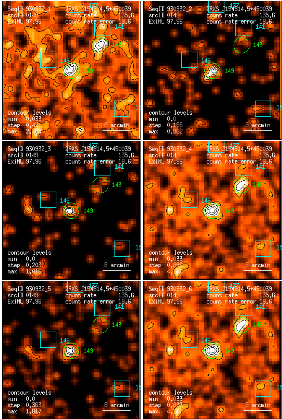
Figure 149: RASS 930932: detection 0149: band rate images, Gaussian filter: (1) PSPC channels 11 – 41, (2) 52 – 90, (3) 91 – 201, (4) 11 – 235, (5) 52 – 201, (6) 11 – 201. Broad band rates in counts/ks. Band rate contour levels in counts/ks/arcmin 2 .
