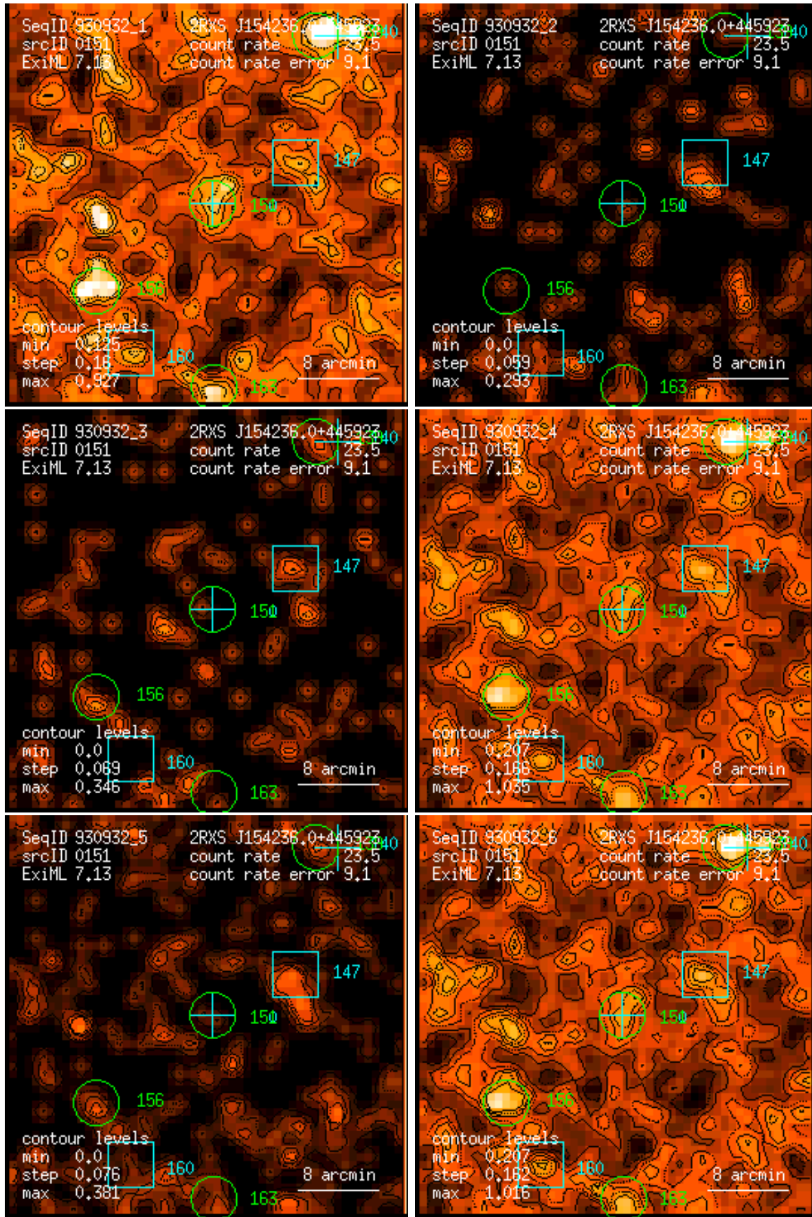
Figure 151: RASS 930932: detection 0151: band rate images, Gaussian filter: (1) PSPC channels 11 – 41, (2) 52 – 90, (3) 91 – 201, (4) 11 – 235, (5) 52 – 201, (6) 11 – 201. Broad band rates in counts/ks. Band rate contour levels in counts/ks/arcmin 2 .
