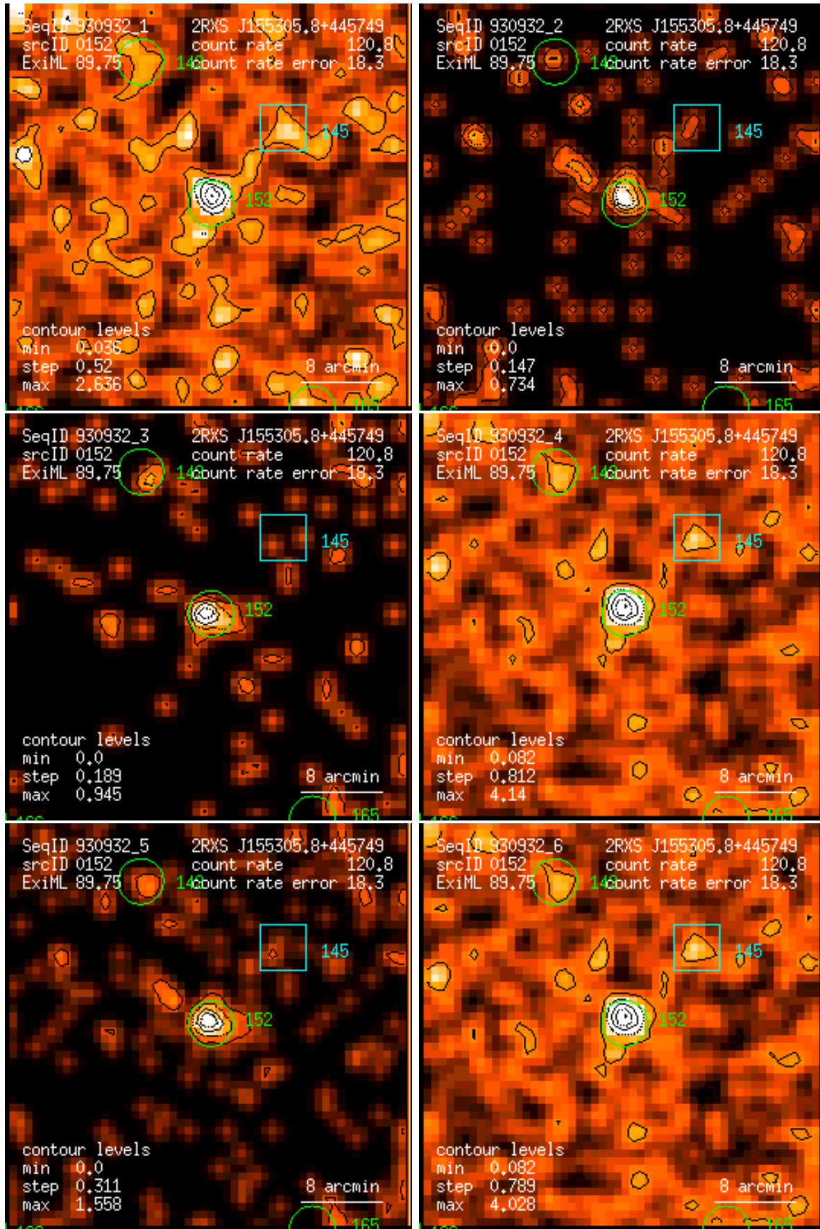
Figure 152: RASS 930932: detection 0152: band rate images, Gaussian filter: (1) PSPC channels 11 – 41, (2) 52 – 90, (3) 91 – 201, (4) 11 – 235, (5) 52 – 201, (6) 11 – 201. Broad band rates in counts/ks. Band rate contour levels in counts/ks/arcmin 2 .
