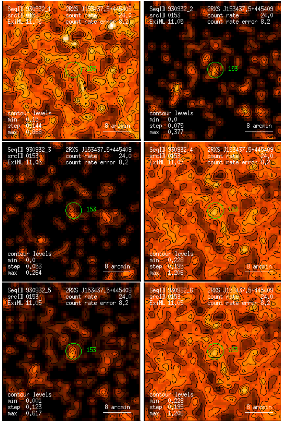
Figure 153: RASS 930932: detection 0153: band rate images, Gaussian filter: (1) PSPC channels 11 – 41, (2) 52 – 90, (3) 91 – 201, (4) 11 – 235, (5) 52 – 201, (6) 11 – 201. Broad band rates in counts/ks. Band rate contour levels in counts/ks/arcmin 2 .
