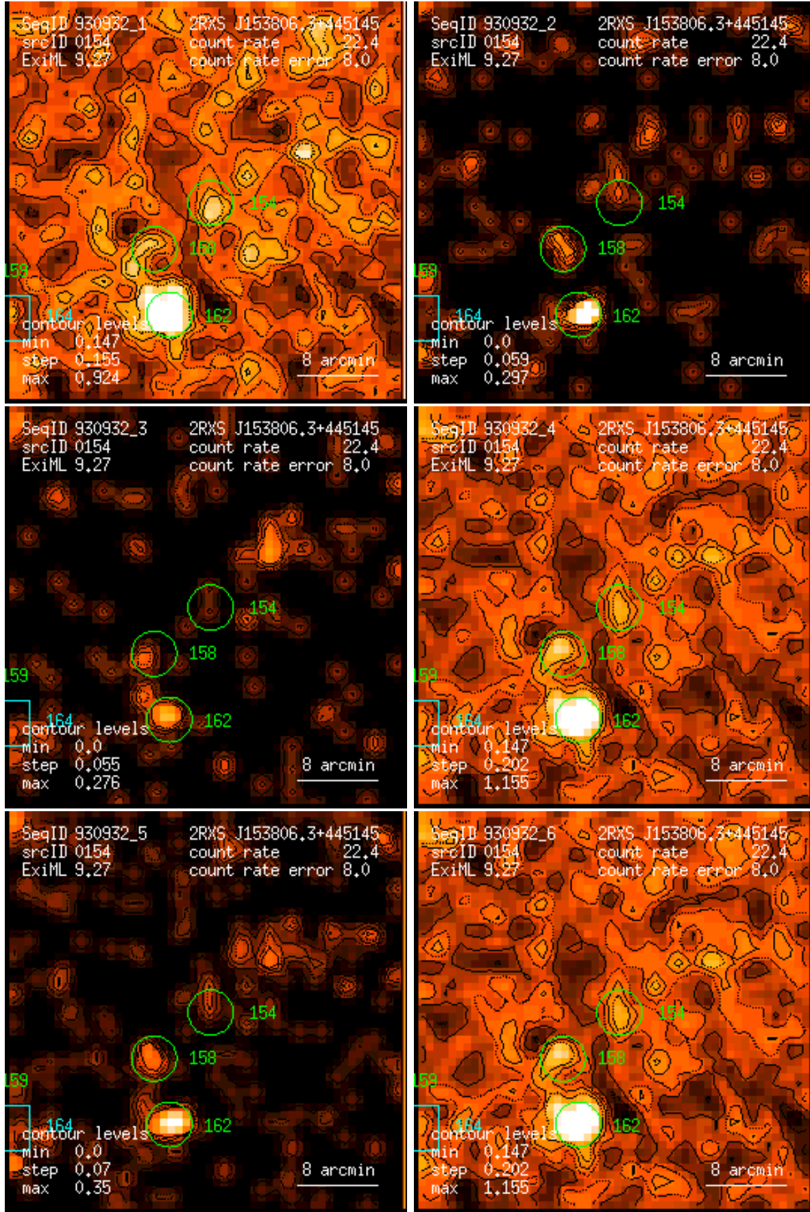
Figure 154: RASS 930932: detection 0154: band rate images, Gaussian filter: (1) PSPC channels 11 – 41, (2) 52 – 90, (3) 91 – 201, (4) 11 – 235, (5) 52 – 201, (6) 11 – 201. Broad band rates in counts/ks. Band rate contour levels in counts/ks/arcmin 2 .
