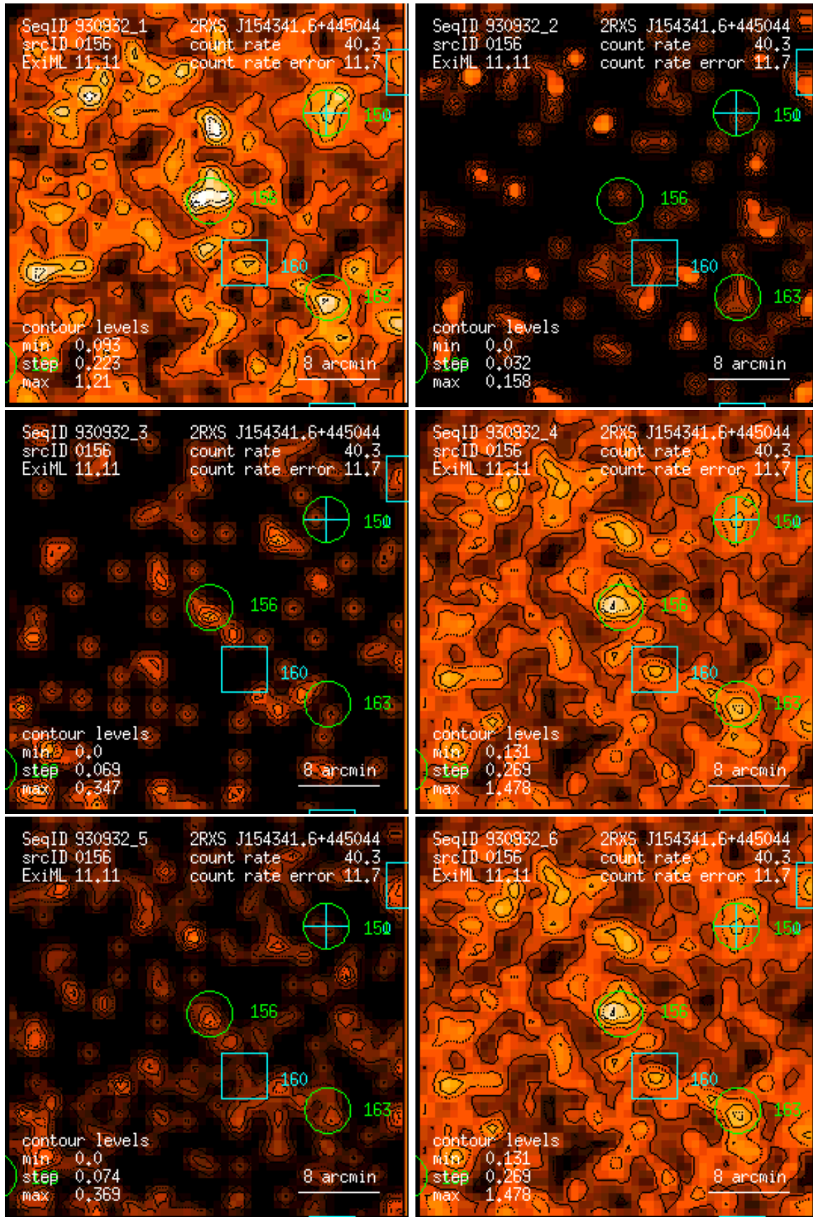
Figure 156: RASS 930932: detection 0156: band rate images, Gaussian filter: (1) PSPC channels 11 – 41, (2) 52 – 90, (3) 91 – 201, (4) 11 – 235, (5) 52 – 201, (6) 11 – 201. Broad band rates in counts/ks. Band rate contour levels in counts/ks/arcmin 2 .
