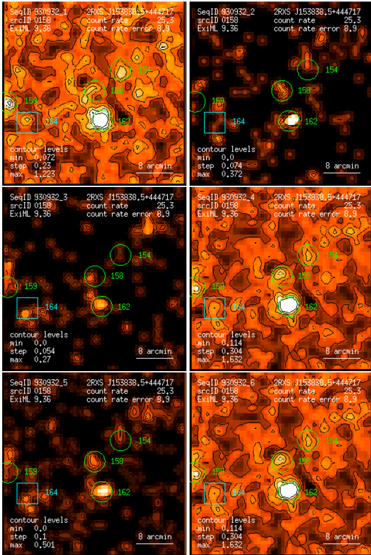
Figure 158: RASS 930932: detection 0158: band rate images, Gaussian filter: (1) PSPC channels 11 – 41, (2) 52 – 90, (3) 91 – 201, (4) 11 – 235, (5) 52 – 201, (6) 11 – 201. Broad band rates in counts/ks. Band rate contour levels in counts/ks/arcmin 2 .
