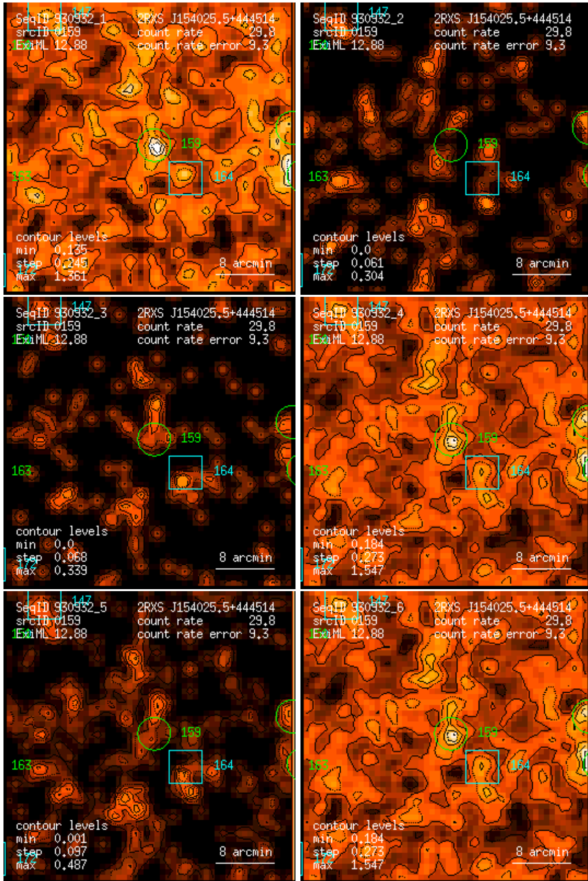
Figure 159: RASS 930932: detection 0159: band rate images, Gaussian filter: (1) PSPC channels 11 – 41, (2) 52 – 90, (3) 91 – 201, (4) 11 – 235, (5) 52 – 201, (6) 11 – 201. Broad band rates in counts/ks. Band rate contour levels in counts/ks/arcmin 2 .
