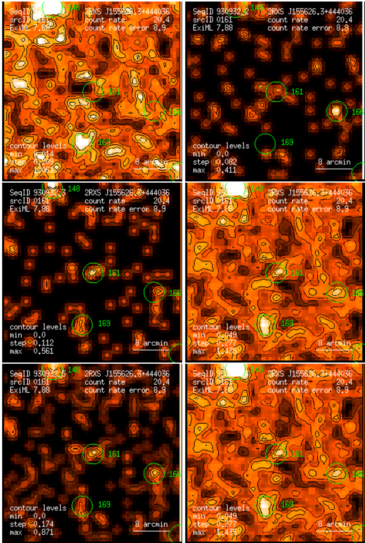
Figure 161: RASS 930932: detection 0161: band rate images, Gaussian filter: (1) PSPC channels 11 – 41, (2) 52 – 90, (3) 91 – 201, (4) 11 – 235, (5) 52 – 201, (6) 11 – 201. Broad band rates in counts/ks. Band rate contour levels in counts/ks/arcmin 2 .
