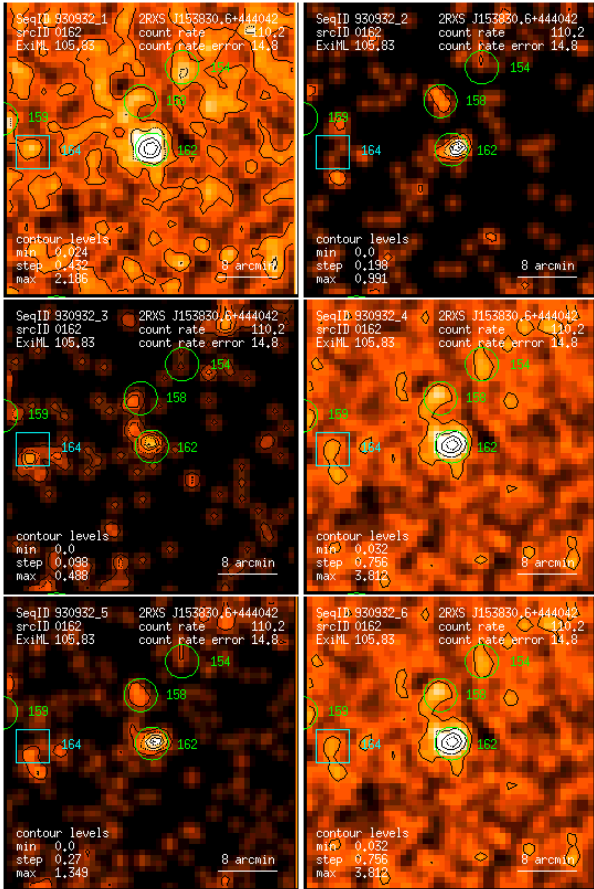
Figure 162: RASS 930932: detection 0162: band rate images, Gaussian filter: (1) PSPC channels 11 – 41, (2) 52 – 90, (3) 91 – 201, (4) 11 – 235, (5) 52 – 201, (6) 11 – 201. Broad band rates in counts/ks. Band rate contour levels in counts/ks/arcmin 2 .
