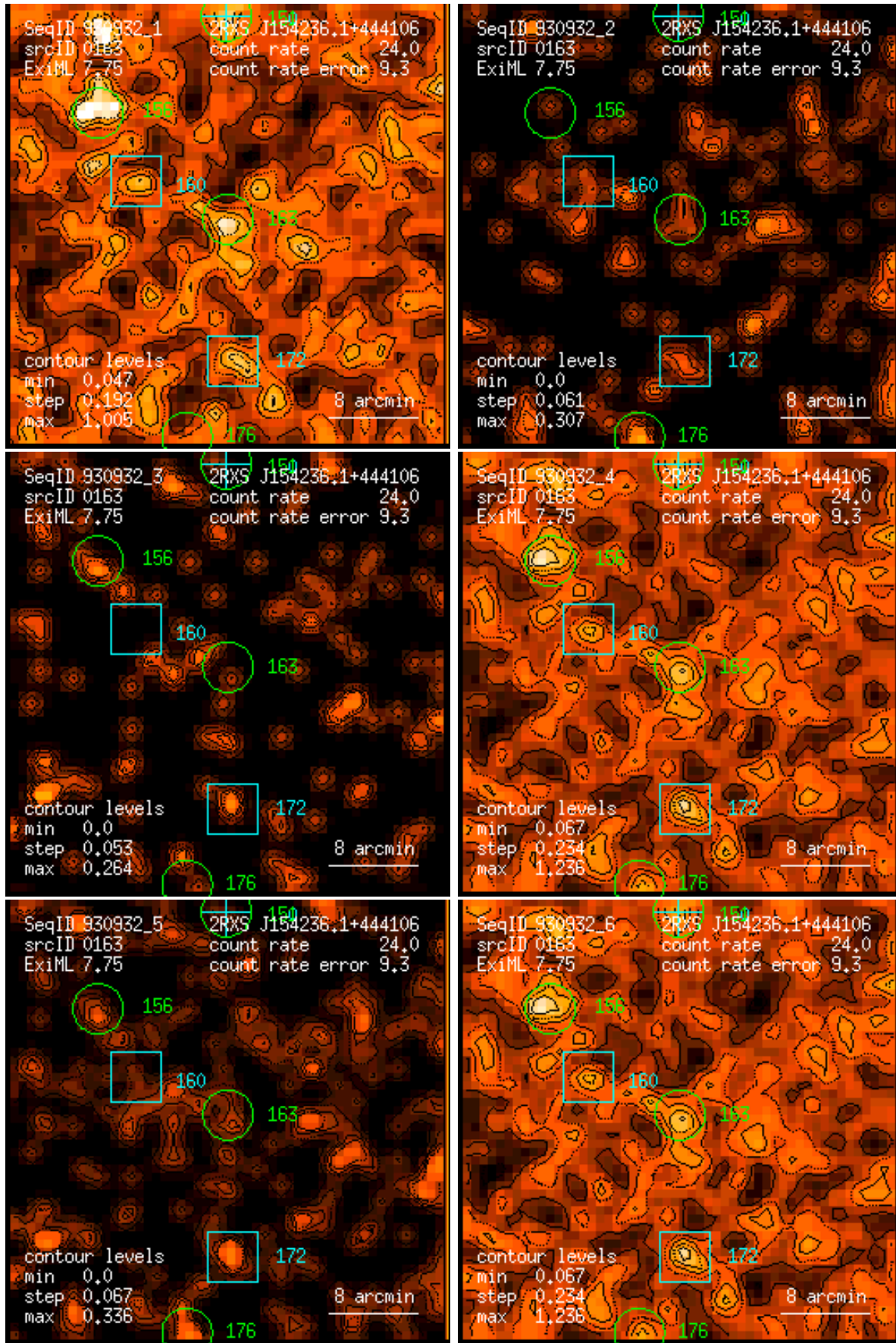
Figure 163: RASS 930932: detection 0163: band rate images, Gaussian filter: (1) PSPC channels 11 – 41, (2) 52 – 90, (3) 91 – 201, (4) 11 – 235, (5) 52 – 201, (6) 11 – 201. Broad band rates in counts/ks. Band rate contour levels in counts/ks/arcmin 2 .
