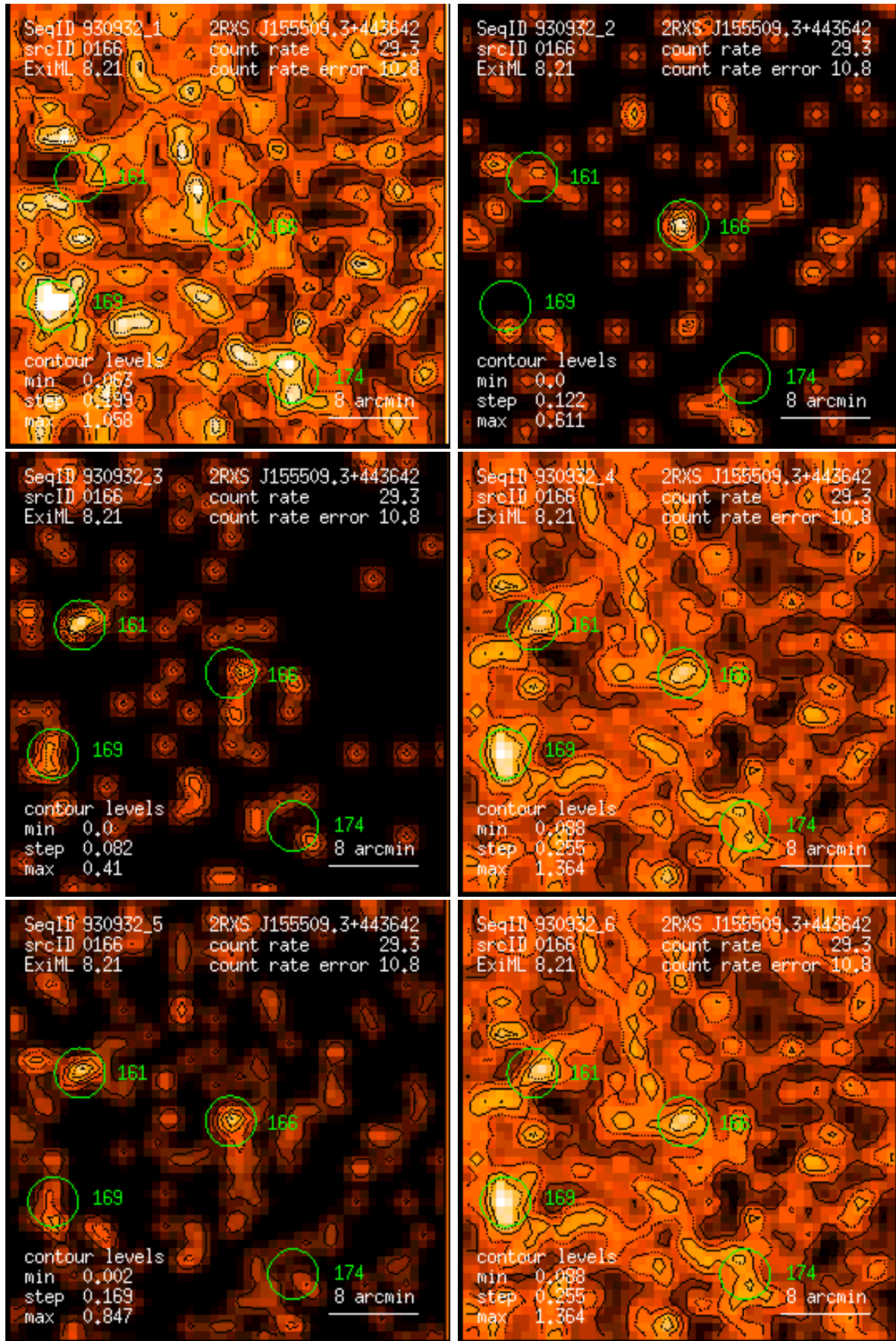
Figure 166: RASS 930932: detection 0166: band rate images, Gaussian filter: (1) PSPC channels 11 – 41, (2) 52 – 90, (3) 91 – 201, (4) 11 – 235, (5) 52 – 201, (6) 11 – 201. Broad band rates in counts/ks. Band rate contour levels in counts/ks/arcmin 2 .
