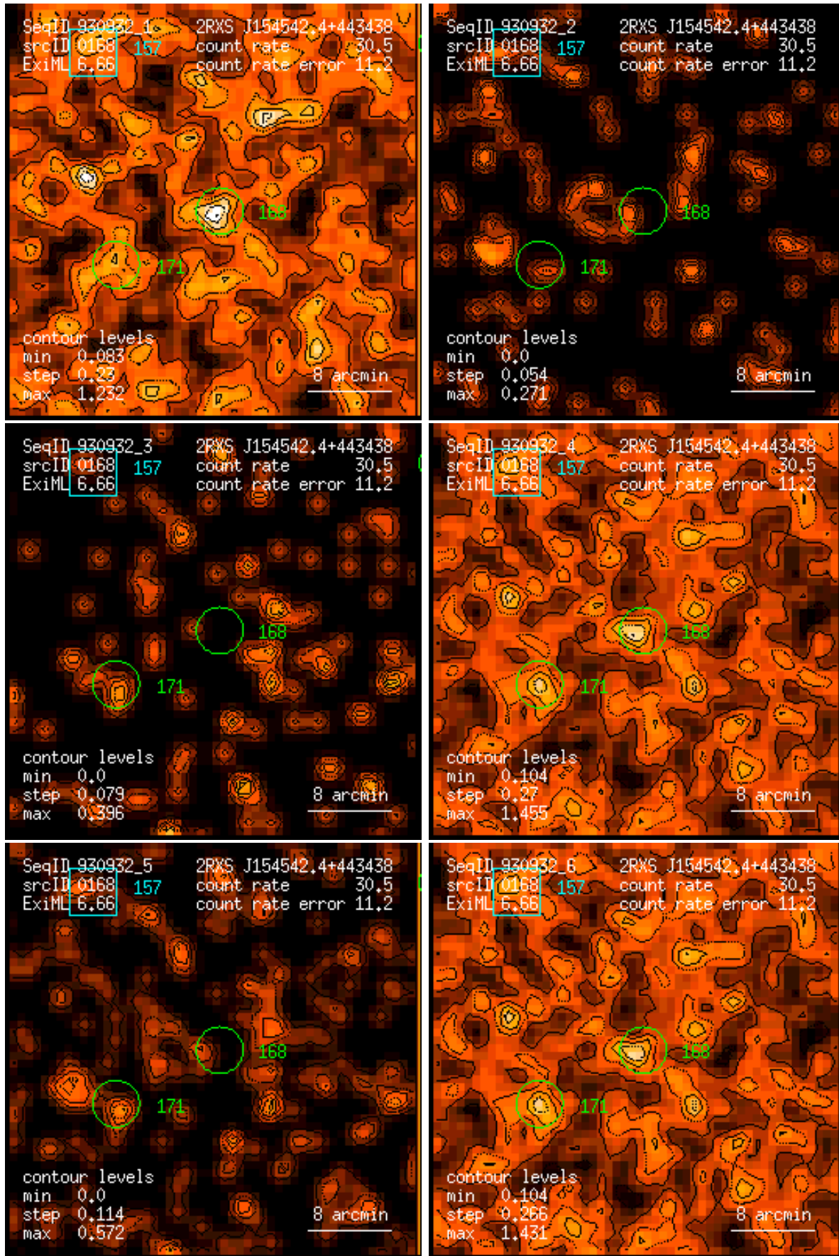
Figure 168: RASS 930932: detection 0168: band rate images, Gaussian filter: (1) PSPC channels 11 – 41, (2) 52 – 90, (3) 91 – 201, (4) 11 – 235, (5) 52 – 201, (6) 11 – 201. Broad band rates in counts/ks. Band rate contour levels in counts/ks/arcmin 2 .
