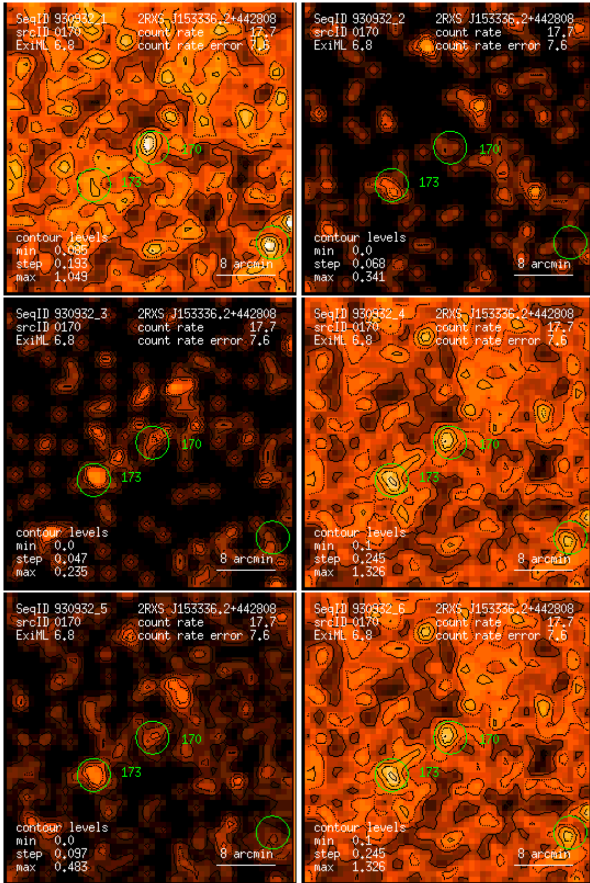
Figure 170: RASS 930932: detection 0170: band rate images, Gaussian filter: (1) PSPC channels 11 – 41, (2) 52 – 90, (3) 91 – 201, (4) 11 – 235, (5) 52 – 201, (6) 11 – 201. Broad band rates in counts/ks. Band rate contour levels in counts/ks/arcmin 2 .
