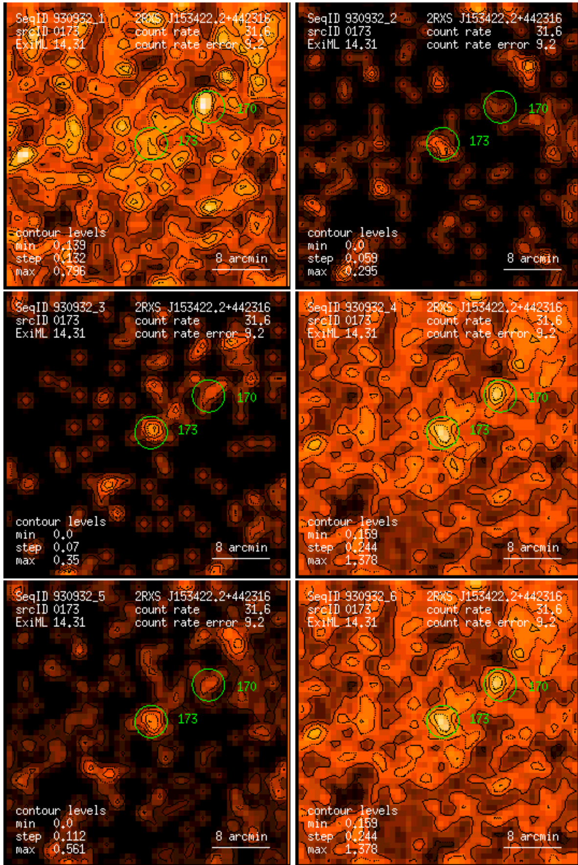
Figure 173: RASS 930932: detection 0173: band rate images, Gaussian filter: (1) PSPC channels 11 – 41, (2) 52 – 90, (3) 91 – 201, (4) 11 – 235, (5) 52 – 201, (6) 11 – 201. Broad band rates in counts/ks. Band rate contour levels in counts/ks/arcmin 2 .
