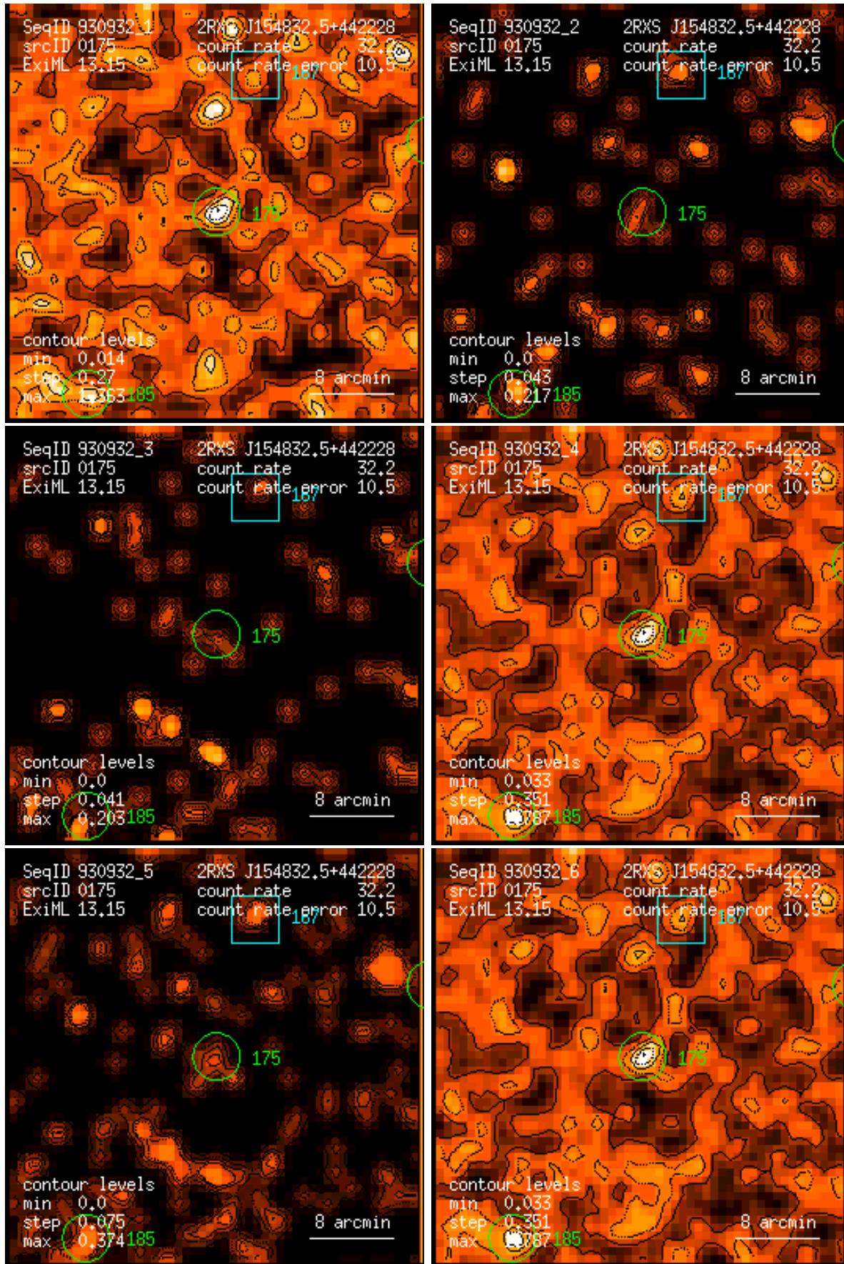
Figure 175: RASS 930932: detection 0175: band rate images, Gaussian filter: (1) PSPC channels 11 – 41, (2) 52 – 90, (3) 91 – 201, (4) 11 – 235, (5) 52 – 201, (6) 11 – 201. Broad band rates in counts/ks. Band rate contour levels in counts/ks/arcmin 2 .
