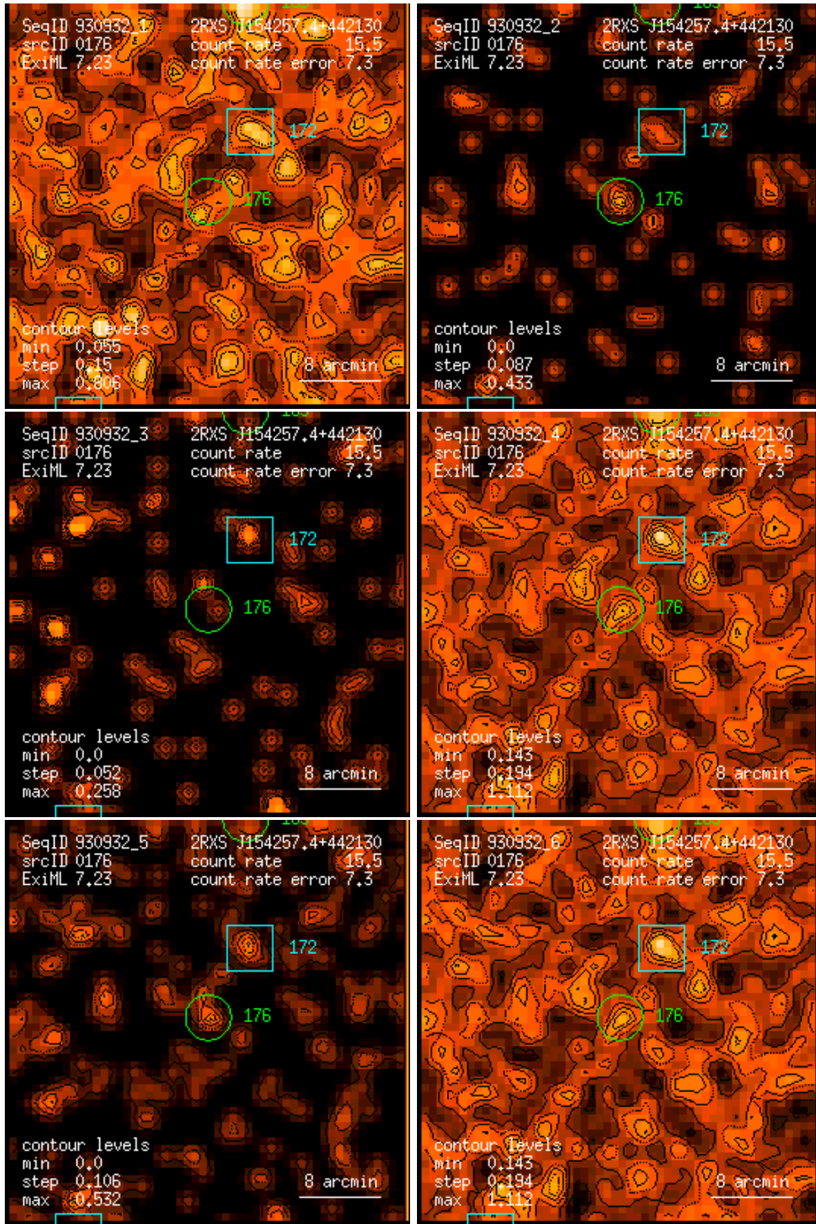
Figure 176: RASS 930932: detection 0176: band rate images, Gaussian filter: (1) PSPC channels 11 – 41, (2) 52 – 90, (3) 91 – 201, (4) 11 – 235, (5) 52 – 201, (6) 11 – 201. Broad band rates in counts/ks. Band rate contour levels in counts/ks/arcmin 2 .
