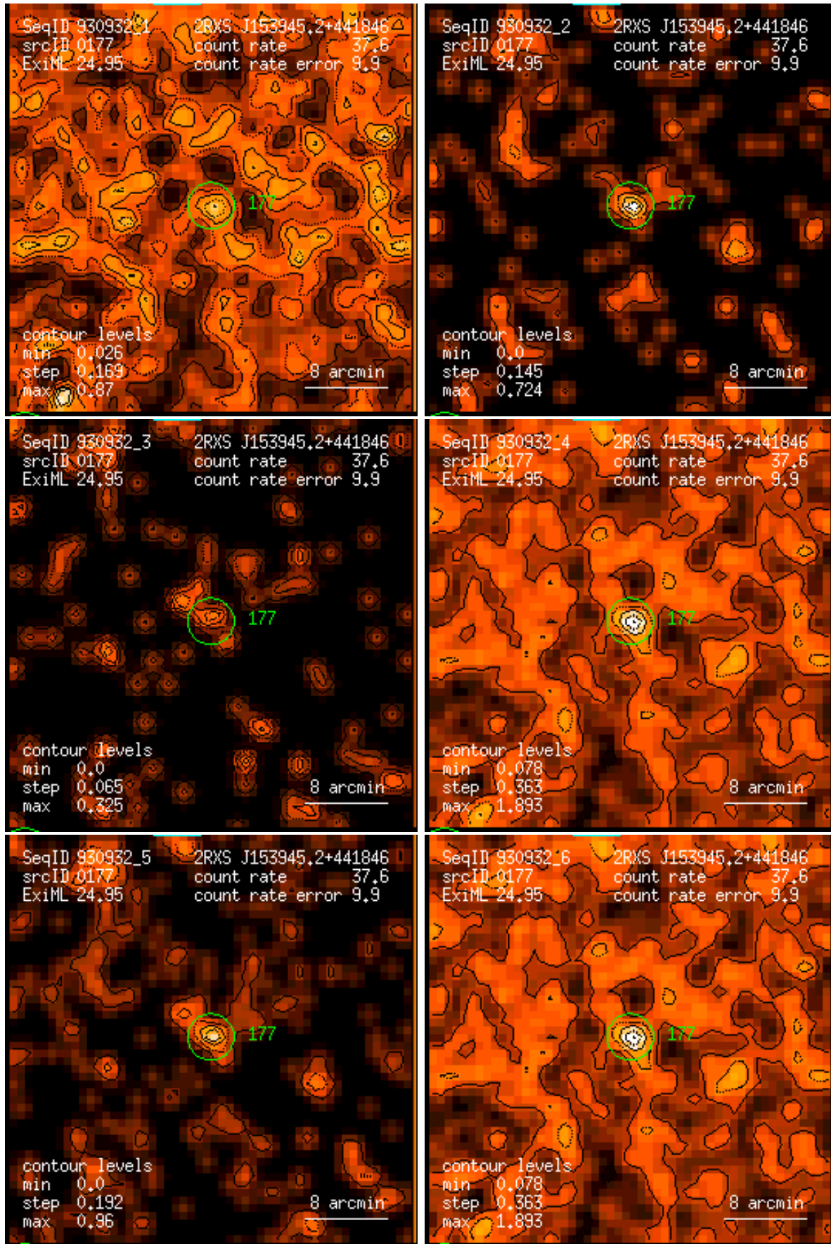
Figure 177: RASS 930932: detection 0177: band rate images, Gaussian filter: (1) PSPC channels 11 – 41, (2) 52 – 90, (3) 91 – 201, (4) 11 – 235, (5) 52 – 201, (6) 11 – 201. Broad band rates in counts/ks. Band rate contour levels in counts/ks/arcmin 2 .
