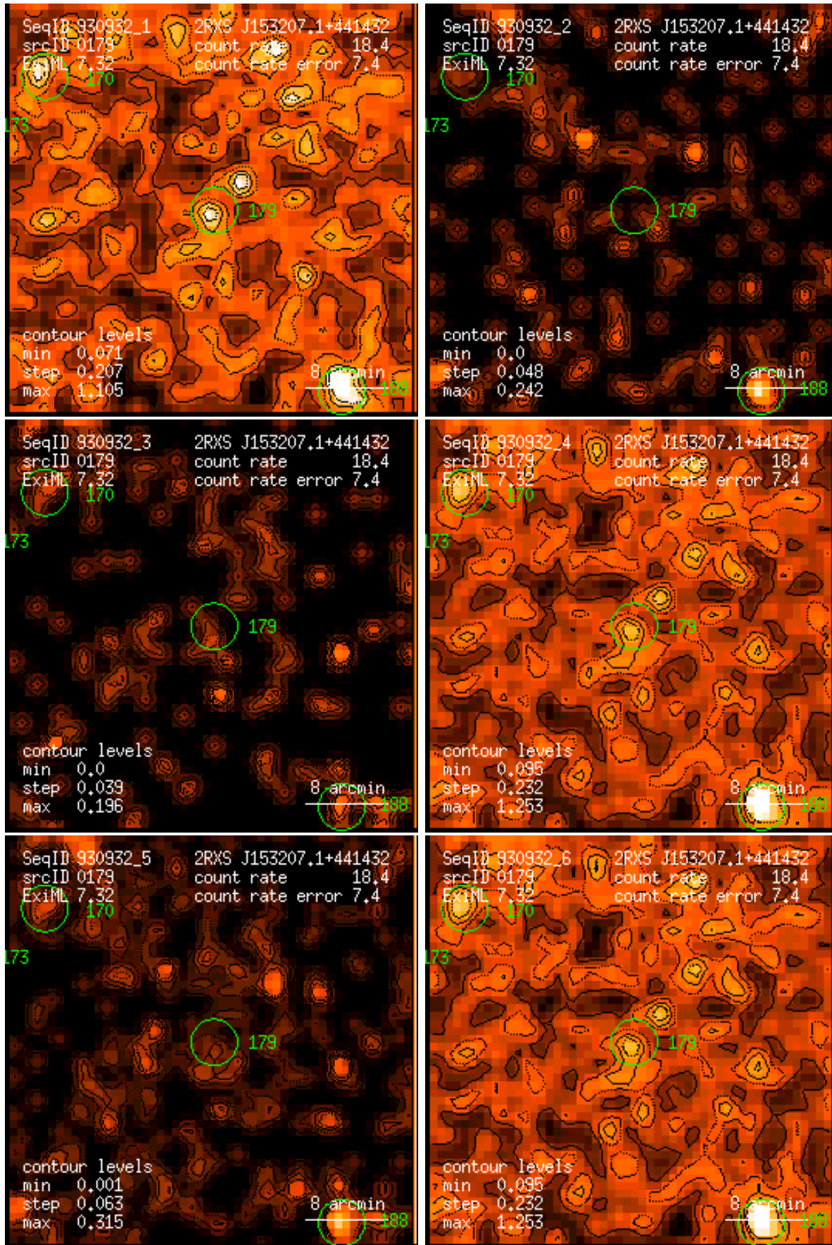
Figure 179: RASS 930932: detection 0179: band rate images, Gaussian filter: (1) PSPC channels 11 – 41, (2) 52 – 90, (3) 91 – 201, (4) 11 – 235, (5) 52 – 201, (6) 11 – 201. Broad band rates in counts/ks. Band rate contour levels in counts/ks/arcmin 2 .
