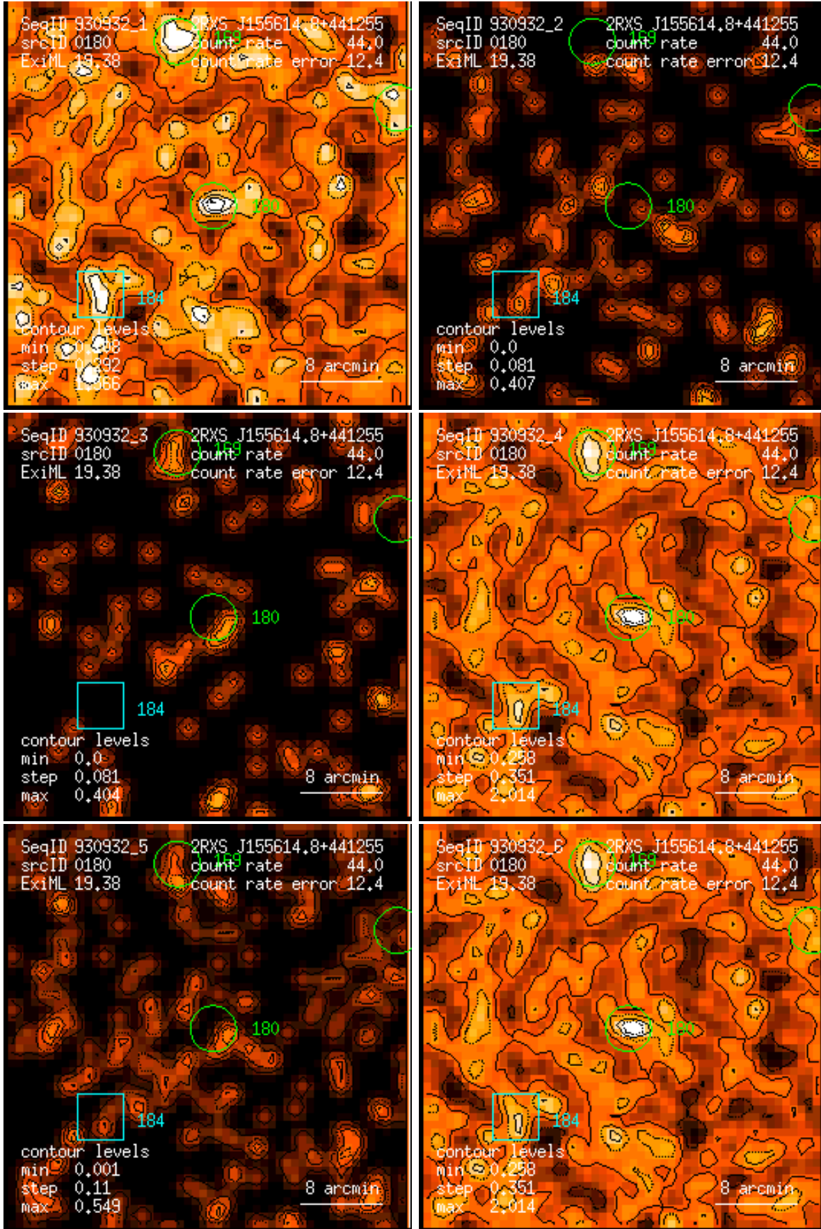
Figure 180: RASS 930932: detection 0180: band rate images, Gaussian filter: (1) PSPC channels 11 – 41, (2) 52 – 90, (3) 91 – 201, (4) 11 – 235, (5) 52 – 201, (6) 11 – 201. Broad band rates in counts/ks. Band rate contour levels in counts/ks/arcmin 2 .
