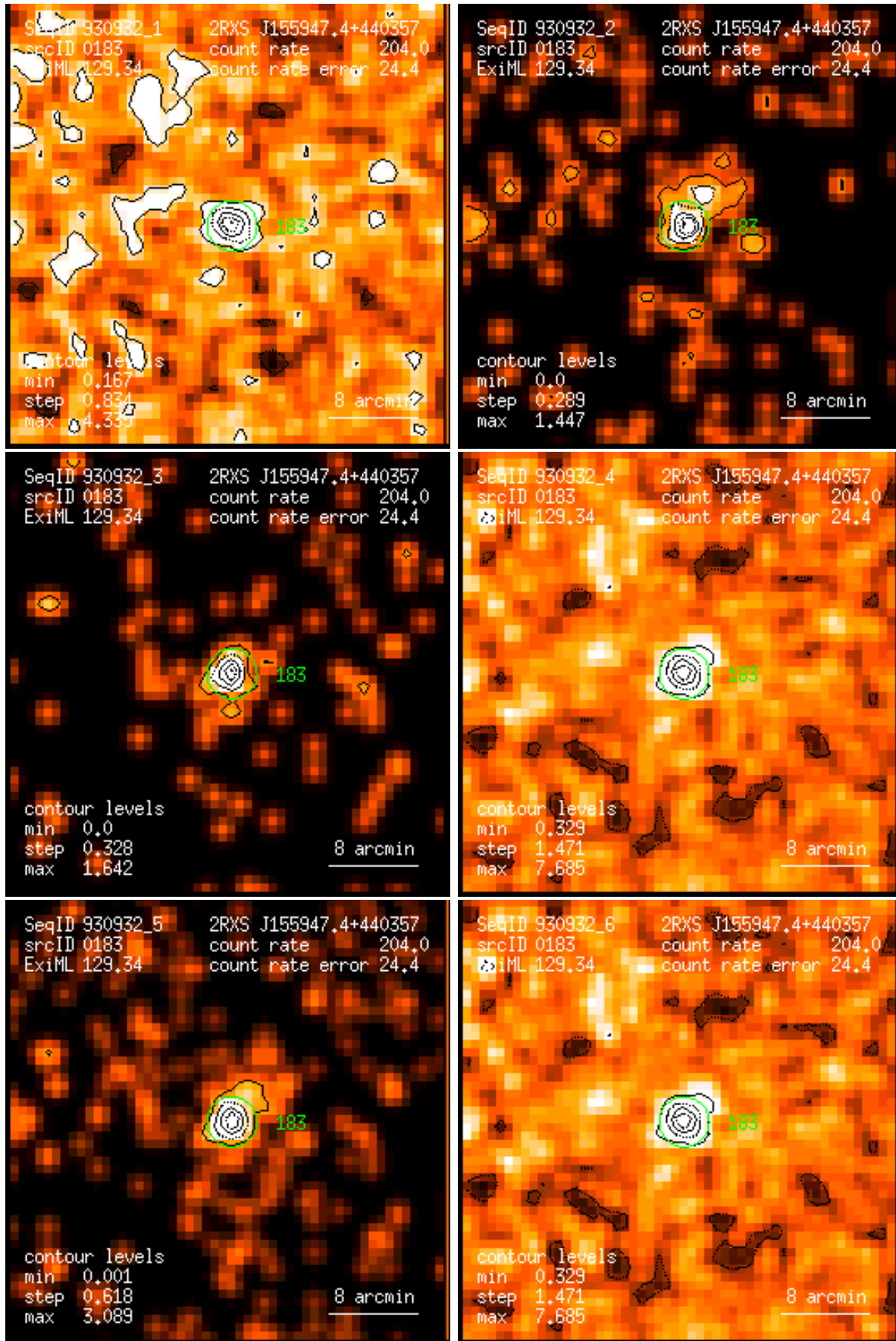
Figure 183: RASS 930932: detection 0183: band rate images, Gaussian filter: (1) PSPC channels 11 – 41, (2) 52 – 90, (3) 91 – 201, (4) 11 – 235, (5) 52 – 201, (6) 11 – 201. Broad band rates in counts/ks. Band rate contour levels in counts/ks/arcmin 2 .
