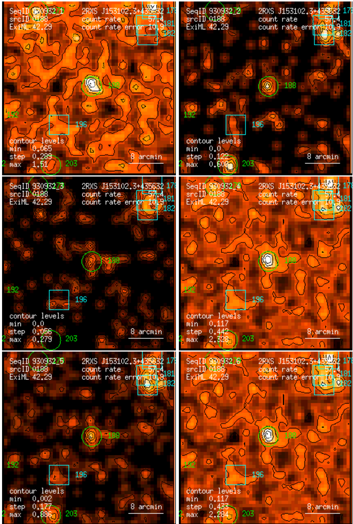
Figure 188: RASS 930932: detection 0188: band rate images, Gaussian filter: (1) PSPC channels 11 – 41, (2) 52 – 90, (3) 91 – 201, (4) 11 – 235, (5) 52 – 201, (6) 11 – 201. Broad band rates in counts/ks. Band rate contour levels in counts/ks/arcmin 2 .
