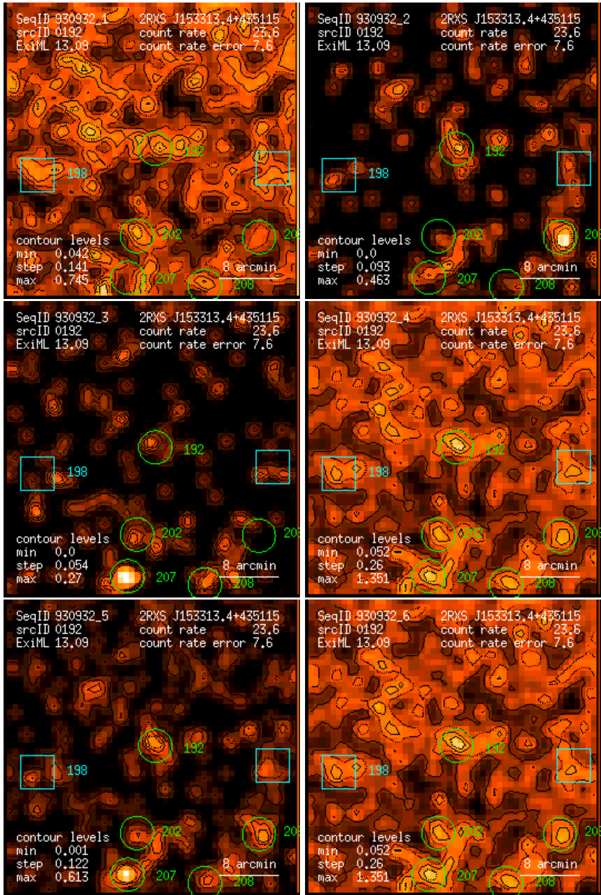
Figure 192: RASS 930932: detection 0192: band rate images, Gaussian filter: (1) PSPC channels 11 – 41, (2) 52 – 90, (3) 91 – 201, (4) 11 – 235, (5) 52 – 201, (6) 11 – 201. Broad band rates in counts/ks. Band rate contour levels in counts/ks/arcmin 2 .
