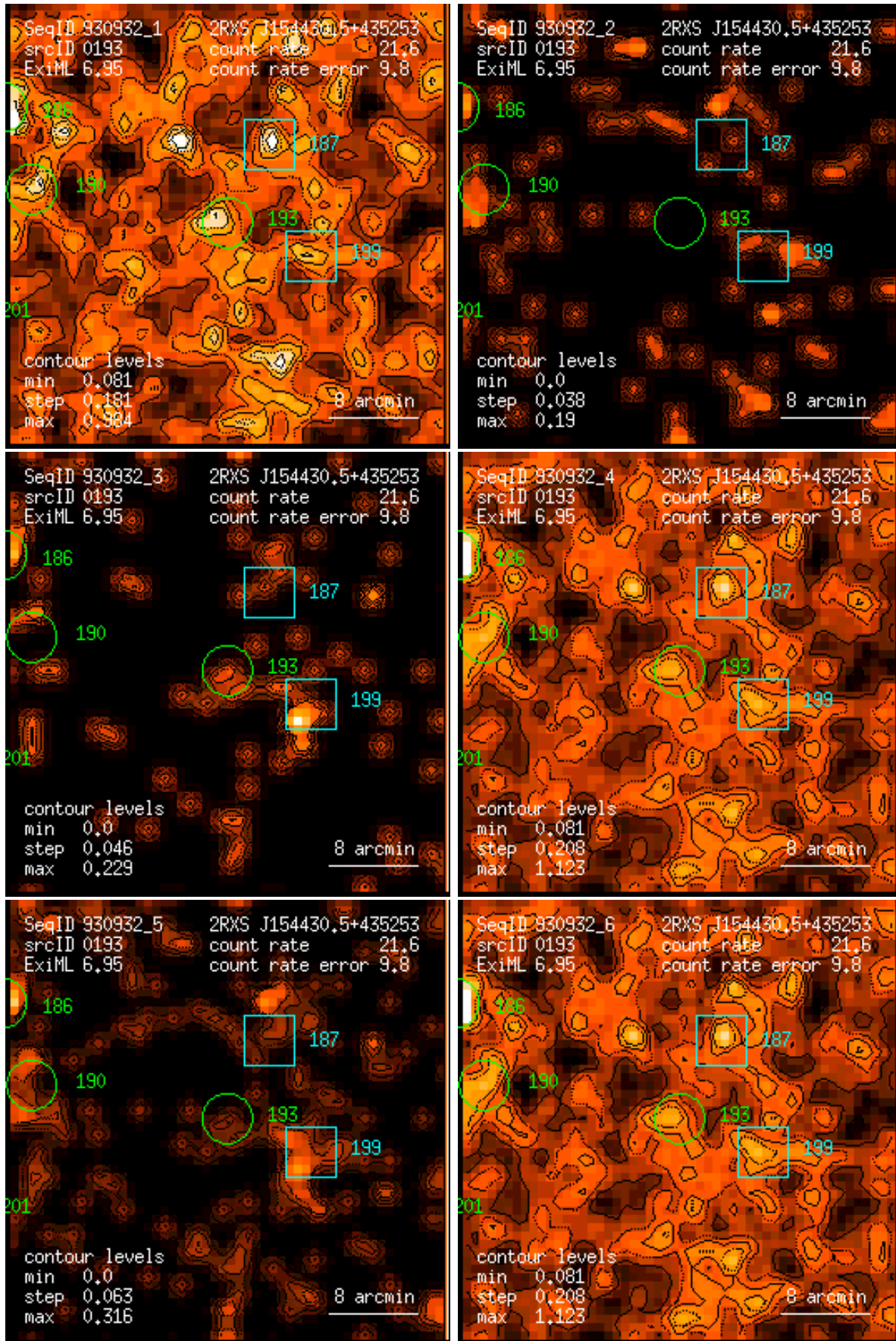
Figure 193: RASS 930932: detection 0193: band rate images, Gaussian filter: (1) PSPC channels 11 – 41, (2) 52 – 90, (3) 91 – 201, (4) 11 – 235, (5) 52 – 201, (6) 11 – 201. Broad band rates in counts/ks. Band rate contour levels in counts/ks/arcmin 2 .
