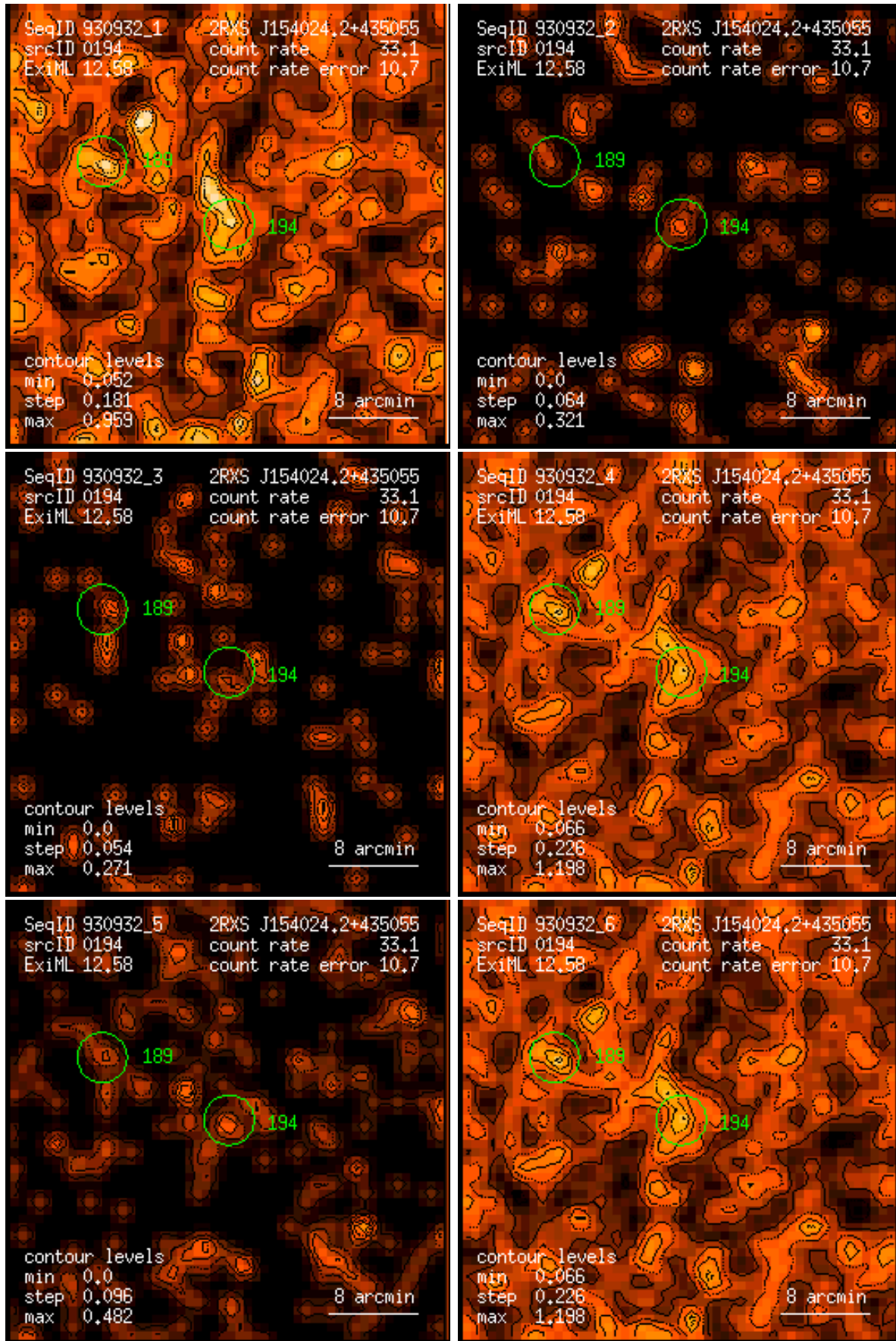
Figure 194: RASS 930932: detection 0194: band rate images, Gaussian filter: (1) PSPC channels 11 – 41, (2) 52 – 90, (3) 91 – 201, (4) 11 – 235, (5) 52 – 201, (6) 11 – 201. Broad band rates in counts/ks. Band rate contour levels in counts/ks/arcmin 2 .
