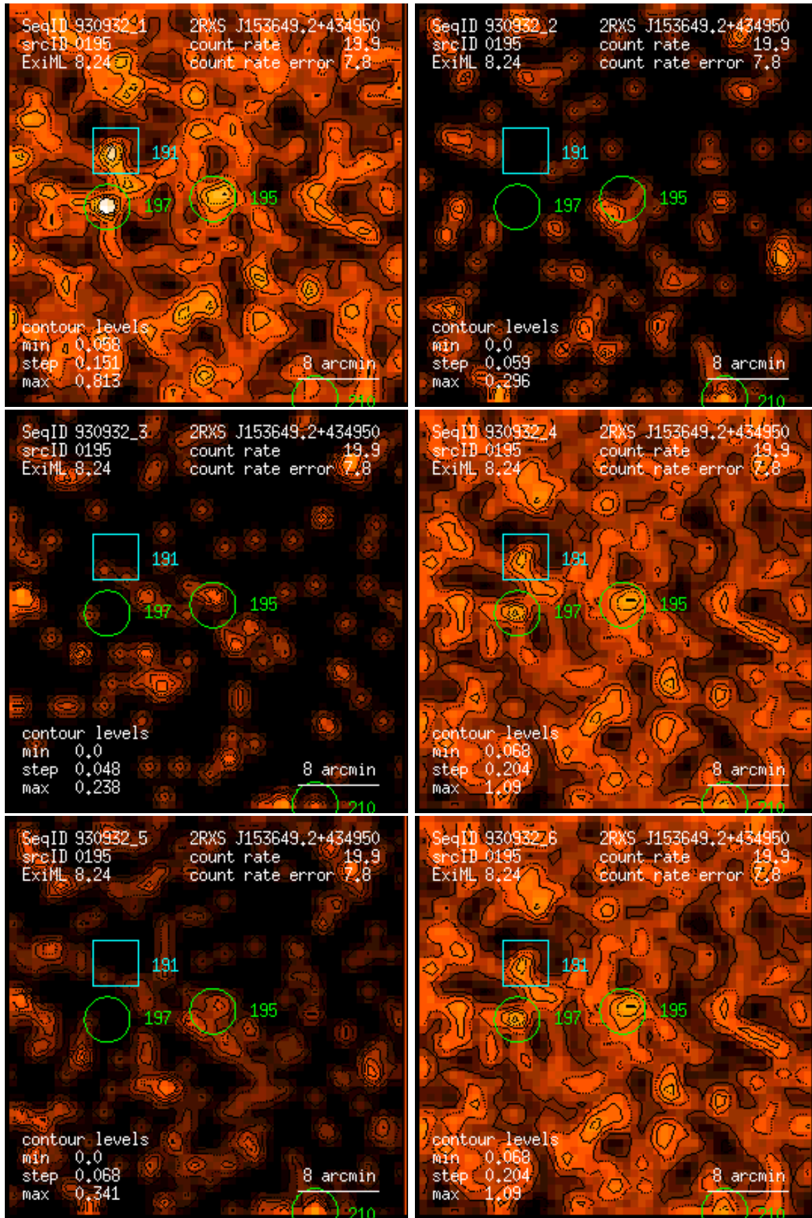
Figure 195: RASS 930932: detection 0195: band rate images, Gaussian filter: (1) PSPC channels 11 – 41, (2) 52 – 90, (3) 91 – 201, (4) 11 – 235, (5) 52 – 201, (6) 11 – 201. Broad band rates in counts/ks. Band rate contour levels in counts/ks/arcmin 2 .
