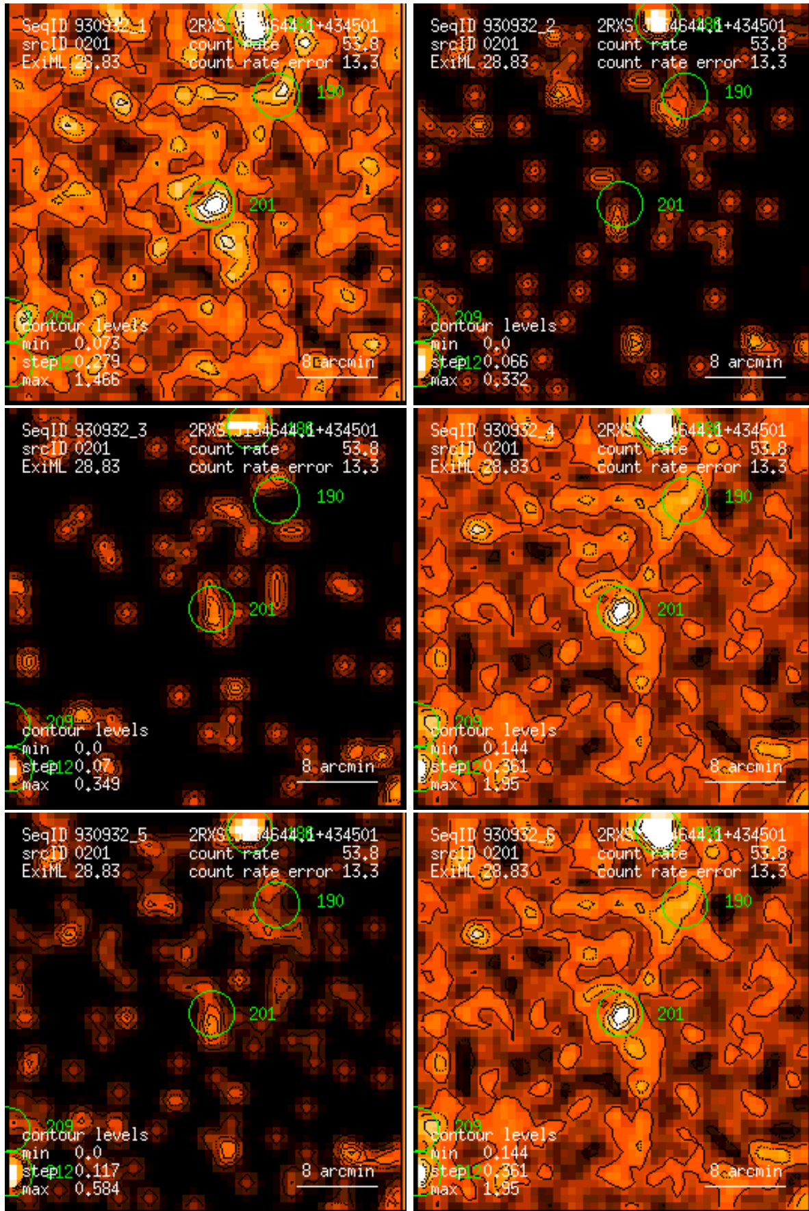
Figure 201: RASS 930932: detection 0201: band rate images, Gaussian filter: (1) PSPC channels 11 – 41, (2) 52 – 90, (3) 91 – 201, (4) 11 – 235, (5) 52 – 201, (6) 11 – 201. Broad band rates in counts/ks. Band rate contour levels in counts/ks/arcmin 2 .
