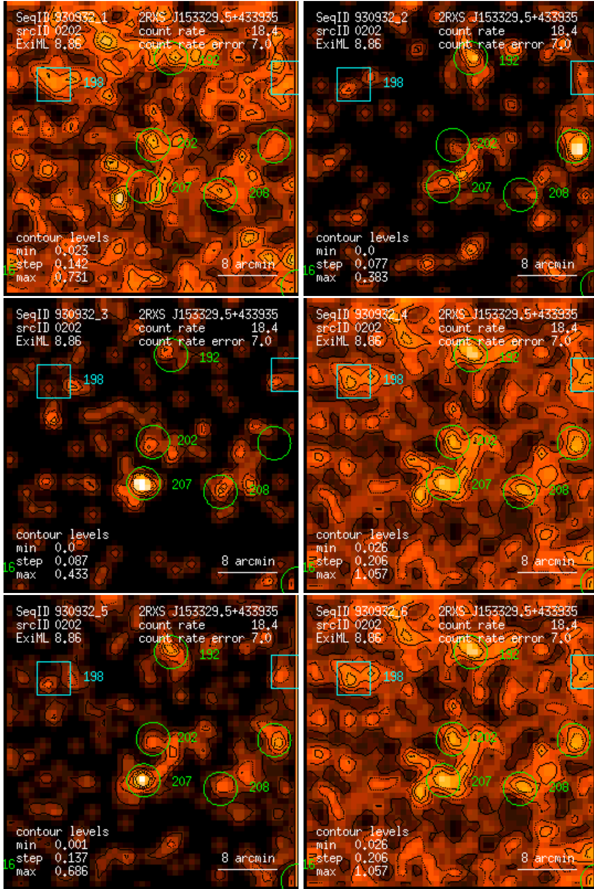
Figure 202: RASS 930932: detection 0202: band rate images, Gaussian filter: (1) PSPC channels 11 – 41, (2) 52 – 90, (3) 91 – 201, (4) 11 – 235, (5) 52 – 201, (6) 11 – 201. Broad band rates in counts/ks. Band rate contour levels in counts/ks/arcmin 2 .
