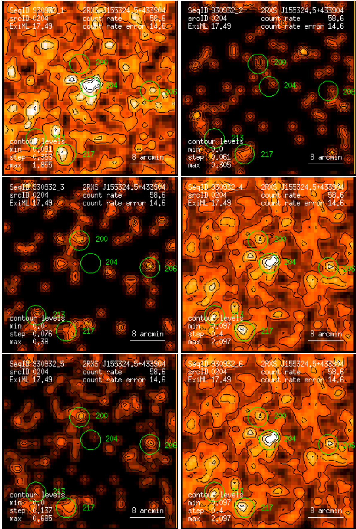
Figure 204: RASS 930932: detection 0204: band rate images, Gaussian filter: (1) PSPC channels 11 – 41, (2) 52 – 90, (3) 91 – 201, (4) 11 – 235, (5) 52 – 201, (6) 11 – 201. Broad band rates in counts/ks. Band rate contour levels in counts/ks/arcmin 2 .
