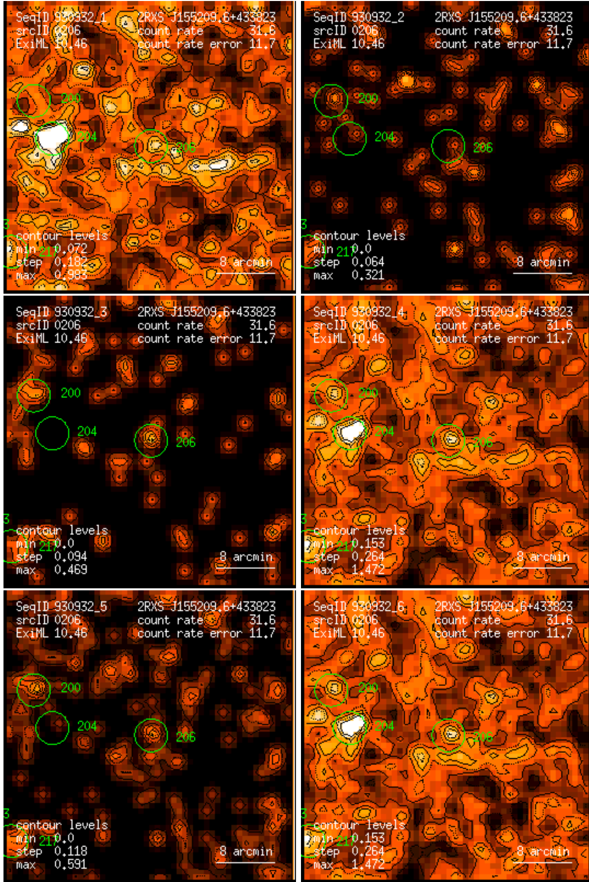
Figure 206: RASS 930932: detection 0206: band rate images, Gaussian filter: (1) PSPC channels 11 – 41, (2) 52 – 90, (3) 91 – 201, (4) 11 – 235, (5) 52 – 201, (6) 11 – 201. Broad band rates in counts/ks. Band rate contour levels in counts/ks/arcmin 2 .
