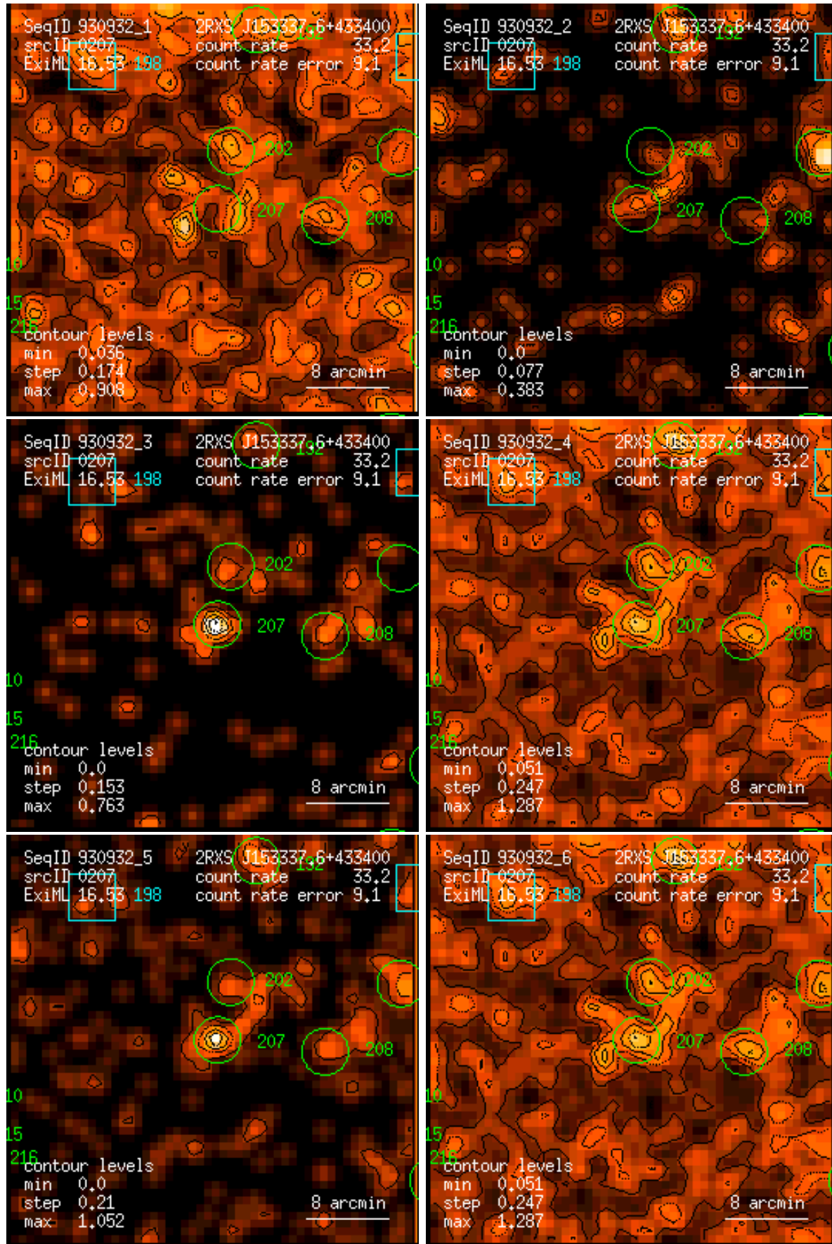
Figure 207: RASS 930932: detection 0207: band rate images, Gaussian filter: (1) PSPC channels 11 – 41, (2) 52 – 90, (3) 91 – 201, (4) 11 – 235, (5) 52 – 201, (6) 11 – 201. Broad band rates in counts/ks. Band rate contour levels in counts/ks/arcmin 2 .
