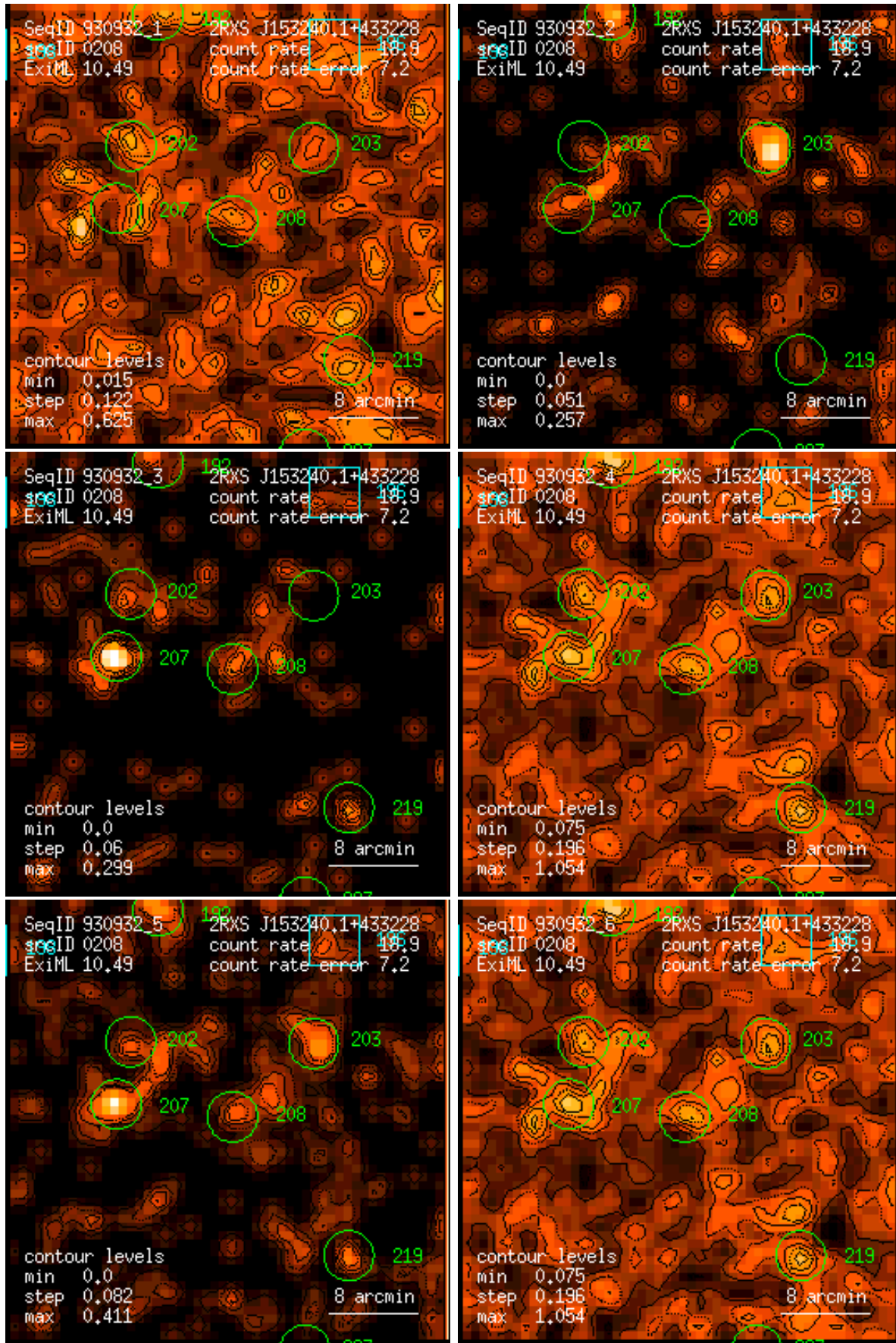
Figure 208: RASS 930932: detection 0208: band rate images, Gaussian filter: (1) PSPC channels 11 – 41, (2) 52 – 90, (3) 91 – 201, (4) 11 – 235, (5) 52 – 201, (6) 11 – 201. Broad band rates in counts/ks. Band rate contour levels in counts/ks/arcmin 2 .
