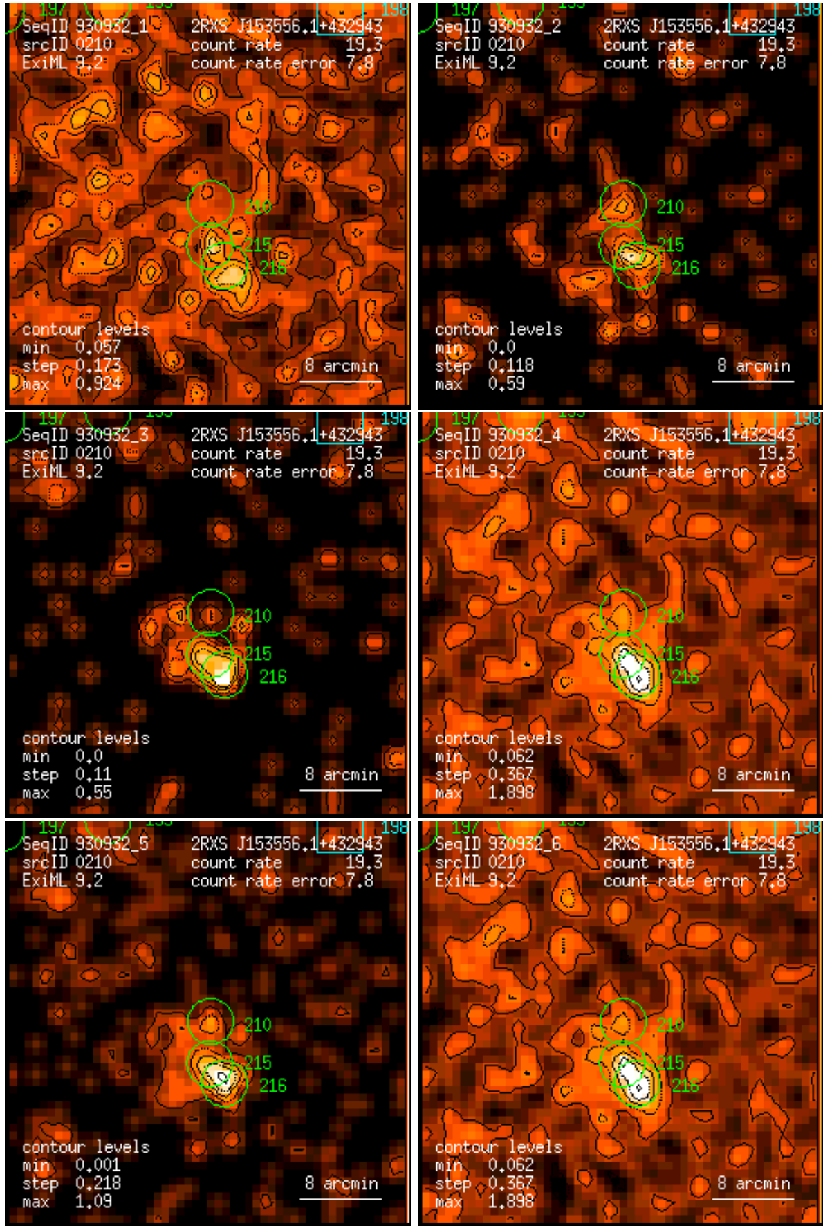
Figure 210: RASS 930932: detection 0210: band rate images, Gaussian filter: (1) PSPC channels 11 – 41, (2) 52 – 90, (3) 91 – 201, (4) 11 – 235, (5) 52 – 201, (6) 11 – 201. Broad band rates in counts/ks. Band rate contour levels in counts/ks/arcmin 2 .
